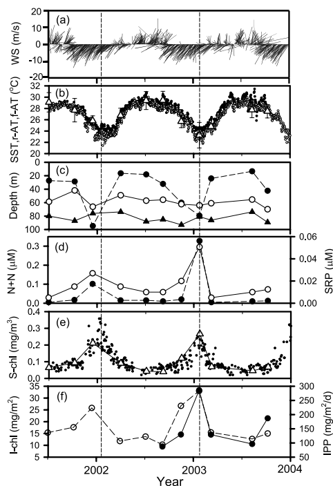
Figure 2. Variations in (a) wind speed (WS) and wind vector, (b) sea surface temperature (SST, ●), remotely sensed air temperature (r-AT, ○) and field observed temperature (f-AT, Δ), (c) mixed layer depth (MLD, ●), top of nutricline depth (TND, ○) and euphotic zone depth (EZD, ▲), (d) averaged mixed-layer (N+N) (●) and SRP (○) concentrations, (e) SeaWiFS-derived (●) and field observed S-chl (Δ), and (f) I-chl (○), and IPP (●) between June 2001 and Dec. 2004. The vertical dashed lines indicate the times of occurrence of maximum S-chl and I-chl in the winter of 2002 and 2003.
