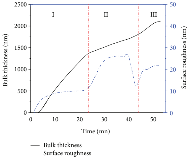
FIGURE 1: Evolution of bulk layer thickness and surface roughness layer thickness—obtained throughout three-stage CIGS growth for 2.0 \mu\text{m} -thick CIGS layer.
