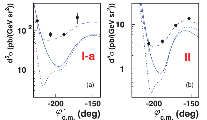
FIG. 14. (Color online) The (ep \rightarrow ep\gamma) cross section for data sets I-a (a) and II (b) at q'_{\text{c.m.}} = 215 \text{ MeV}/c , in-plane ( \theta'_{\text{c.m.}} = 90^\circ ) as a function of \phi'_{\text{c.m.}} . The dashed curve is the DR model calculation, with parameter values as fitted in the experiment. The dotted (respectively, solid) curve is the BH + Born cross section (respectively, plus a first-order GP effect).
