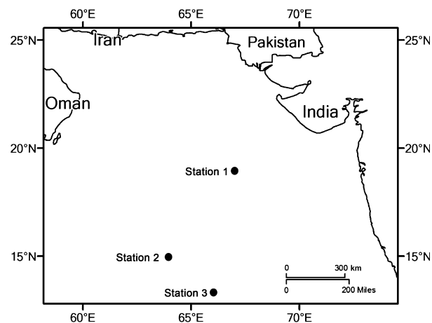
Fig. 1. Map of the Arabian Sea showing the three stations sampled for this study.
