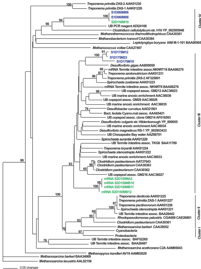
Fig. 4. Neighbor-joining tree of nifH amino acid sequences translated from DNA and cDNA sequences for sequences in Clusters II, III, and IV (Chien & Zinder, 1996). Sequences from this study are identified as described for Fig. 3.
