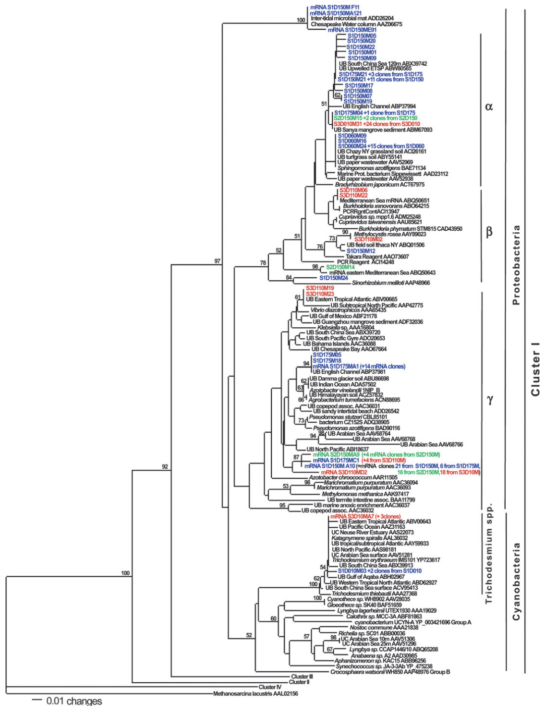
Fig. 3. Neighbor-joining tree of nifH amino acid sequences translated from DNA and cDNA sequences for sequences in Cluster I (Chien & Zinder, 1996). Sequences from this study are identified in color (blue = Station 1, green = Station 2, and red = Station 3), and database sequence names are in black, with accession numbers. Bootstrap values > 50% are indicated. For the new sequences, sequence names (e.g. the sequence from Station 1 at the top of the alpha-proteobacterial cluster in the figure, S1D150M05) provide Station number (S1), depth of sample (D150), and clone number (M05). The cDNA sequences names have the prefix mRNA. UB, uncultured bacterium; UC, uncultured cyanobacterium.
