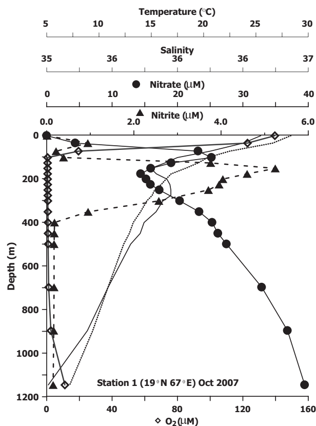
Fig. 2. Vertical distribution of chemical and physical variables at Station 1, showing representative features that characterize the surface, oxycline, and ODZ regions of the water column.
