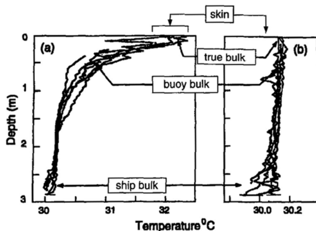
Figure 22. Measurements of temperature profiles in the ocean mixed layer on (a) 13 January 1993 and (b) 4 February 1993. The levels where the skin, true bulk, buoy bulk, and ship bulk SST values are commonly measured are indicated schematically. From Webster et al. [1996]. Copyright 1996 AMS.
