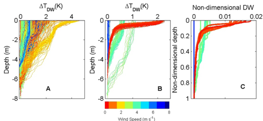
Figure 7. Upper ocean temperature profiles from SkinDeEP. The color of the lines indicates the measured wind speed at the time of the profile. (a) SkinDeEP profiles from 4 to 14 October 1999. (b) Smoothed SkinDeEP profiles from 1200 to 1400 LMT on 4 October and 8–10 October 1999. (c) The profiles from Figure 7b but with the depth normalized by the warm layer depth and normalized heat content. DW, diurnal warming.
