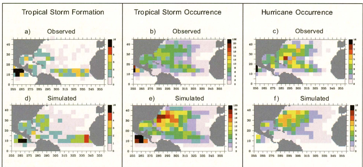
FIG. 3. Maps of observed geographical distribution (1980–2006) of (a) tropical storm formation, (b) tropical storm occurrence, and (c) hurricane occurrence in units of storms per decade within 4° latitude × 5° longitude grid boxes. (d), (e), (f) Simulated distributions for the model ensemble (ModelE).
