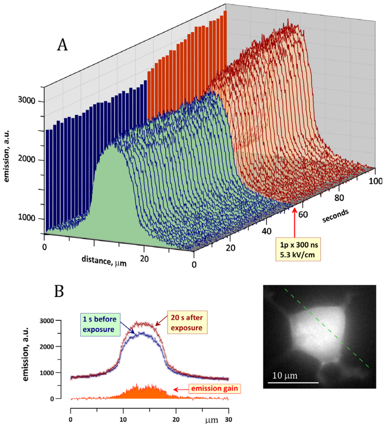
Fig. 4. Lack of localized increase in [Na]_i in the vicinity of the cell plasma membrane following nsPEF exposure. Inset shows a fluorescent image of the cell loaded with 1 \mu\text{m} of Sodium Green. The emission intensity was measured along the dashed line, which connects the tips of nsPEF-delivering electrodes (not shown). A: The emission along the line was measured repeatedly before and after exposure to one 300 ns pulse at 5.3 kV/cm (arrow). Increased emission following exposure reflects the Na^+ influx through the membrane. B: Individual line scans of the emission intensity immediately prior to exposure and 20 s after. The emission gain due to exposure is the arithmetic difference between these two curves. Note
