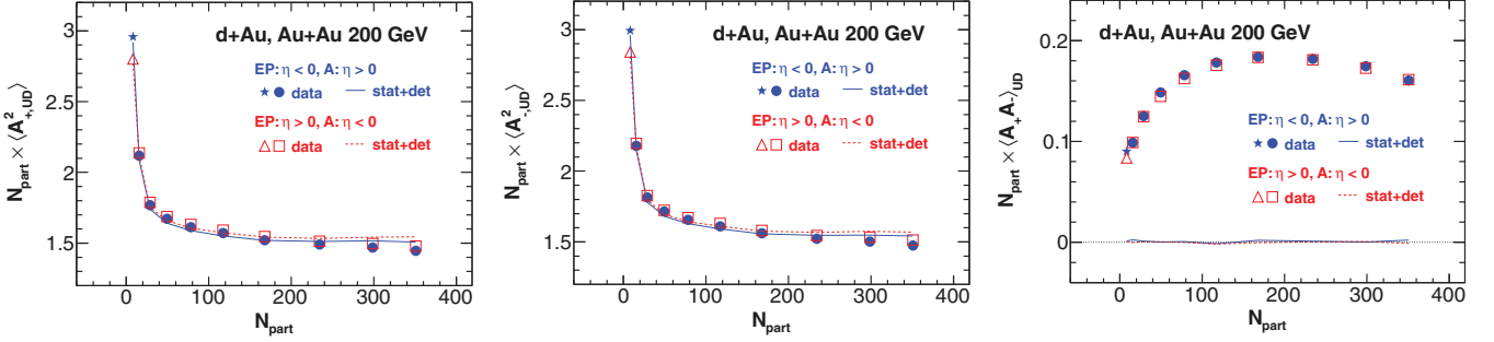
FIG. 20. (Color online) The asymmetry correlations, \langle A_{+,-,UD}^2 \rangle (left panel), \langle A_{-,-,UD}^2 \rangle (middle panel), and \langle A_+ A_- \rangle_{UD} (right panel), multiplied by the number of participants N_{part} , separately for \eta > 0 and \eta < 0 . The star and triangle depict the results from d + Au collisions. The net effects of the statistical fluctuations and detector nonuniformities are shown as the curves. Error bars are statistical only.
