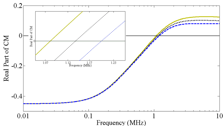
FIG. 8. Effect of cell heterogeneity on CM factor at 0.35 S/m medium conductivity. Continuous, dashed, and dotted lines present maximum, minimum, and average CM factors, respectively.
