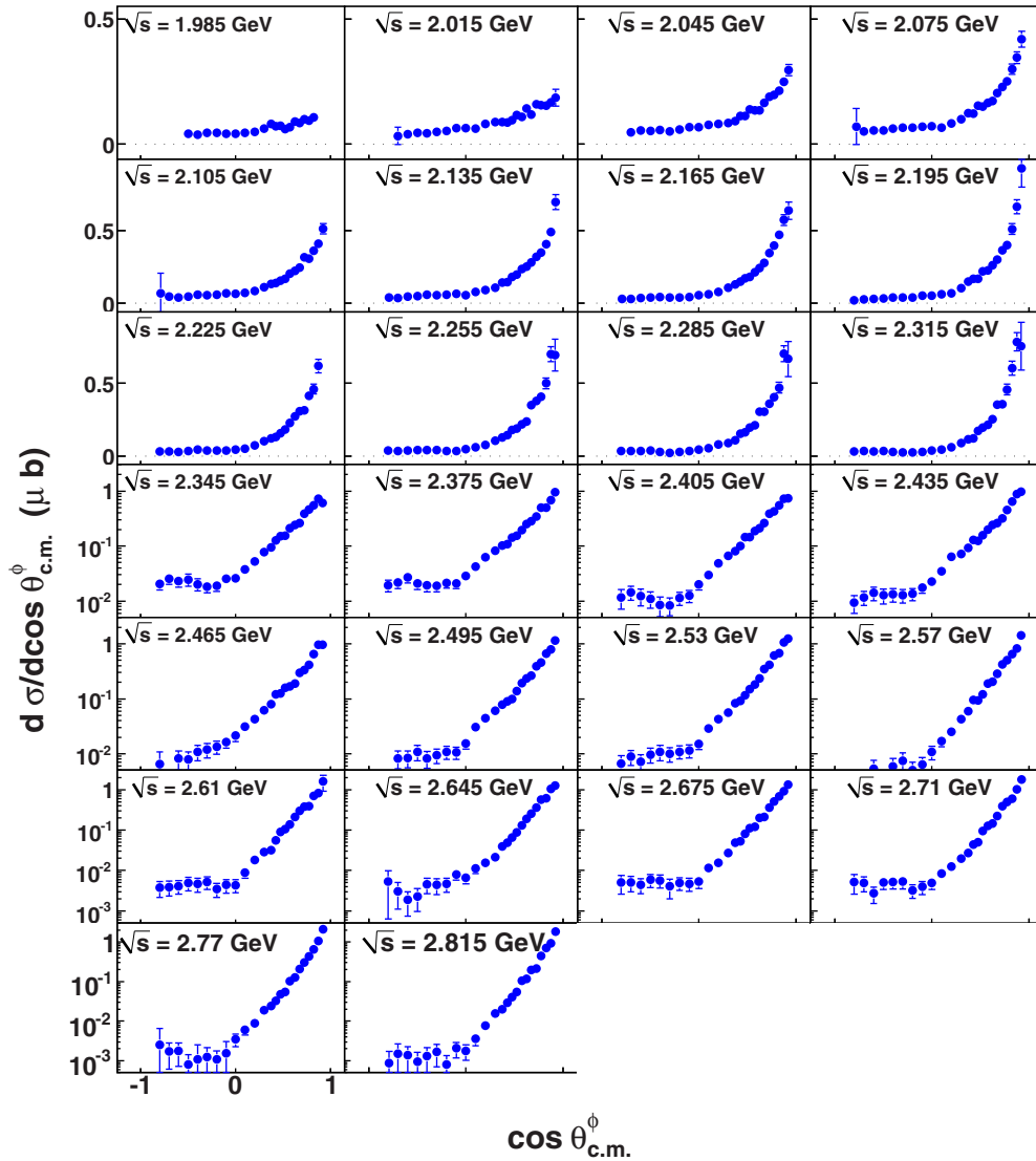
FIG. 15. (Color online) \frac{d\sigma}{d\cos\theta_{\text{c.m.}}} (\mu\text{b}) vs \cos\theta_{\text{c.m.}}^{\phi} : Differential cross section results for the neutral-mode topology. The minimum(maximum) bin-width is 30 MeV(50 MeV) and the bin centroid is printed on the plots. The y-axis range is constant over each horizontal row and is shown in the left-most column for every row. Note that no events are included from the \sqrt{s} \in [2.73, 2.75] GeV region. All error bars represent statistical uncertainties only.
