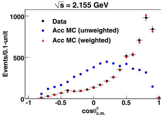
FIG. 9. (Color online) Shown are the \cos \theta_{c.m.}^\phi distributions for the data, accepted Monte Carlo and accepted Monte Carlo weighted by the PWA fit in the \sqrt{s} = 2.155 GeV bin for the charged-two-track topology. Weighting by the fit results brings the weighted Monte Carlo distribution into excellent agreement with the data.
