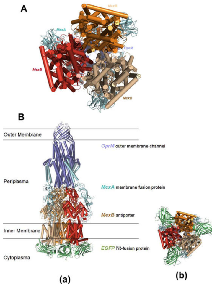
Figure 6. The modeled structures of MexA-(EGFP-MexB)-OprM expressed in the cells ( \Delta MexB): (A) Secondary structure of MexAB-OprM model is constructed based on the coordinates of the data-driven docking model of the multidrug efflux pump (AcrA-AcrB-TolC) from P. aeruginosa . The model shows the location of the MexB N-termini at the cytosolic end of the translocation pore of the transporter with the unstructured loop of the N-termini pointing inward towards the trimeric pore. (B) The EGFP domains were fused to the N-termini of MexB in its trimeric assemblage: (a) stereo side view and (b) bottom view of the structures. Spatial placement of the EGFP domains in the cytosol is limited by potential EGFP to EGFP, or EGFP to MexB clashes in the trimeric configuration. The position and orientation of the N-terminal fused EGFP domains may either partially block the translocation pore or restrict the movement of the individual pump domains, thereby restricting efflux activity.
