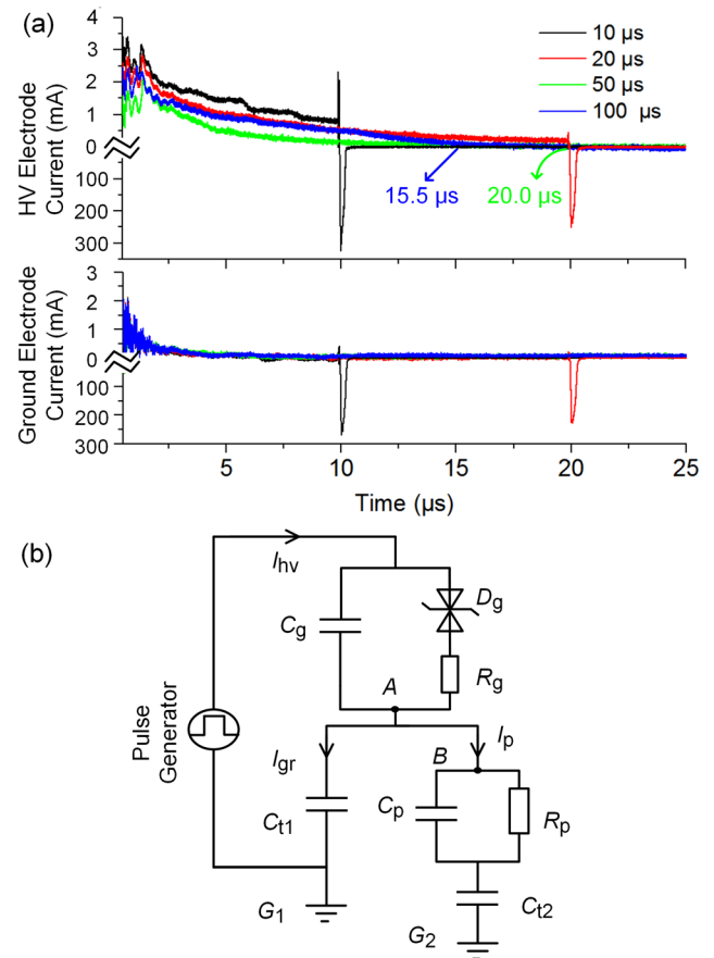
FIG. 4. (a) Discharge currents through the high-voltage electrode and ground electrode for PW = 10, 20, 50, and 100 \mu\text{s} . The waveforms are shown from 0.5 to 25 \mu\text{s} . (b) An equivalent circuit model for pulsed-excited plasmas in a quartz tube.
