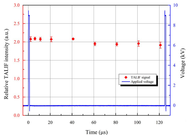
FIG. 25. Time-resolved atomic O TALIF signal of an atmospheric pressure plasma jet during one pulse period. Working gas: premixing 0.9% O 2 with helium. Shielding gas: N 2 . 97
