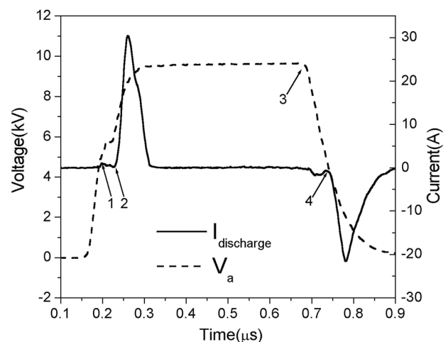
FIG. 10. Current-voltage characteristics of a P-DBD in helium. 24
