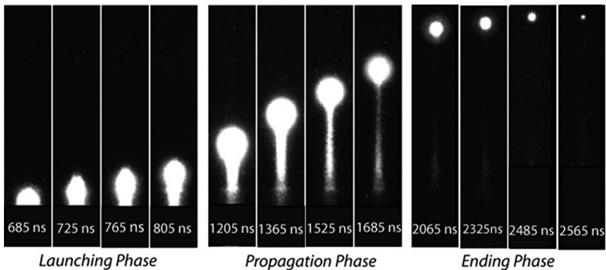
FIG. 17. Plasma bullet velocity versus axial distance showing the three propagation phases (Top figure). The lower figure shows ICCD images of the plasma bullet corresponding to the three propagation phases. Gas: helium at 5 slm; Pulse width: 2 \mu s. 58
