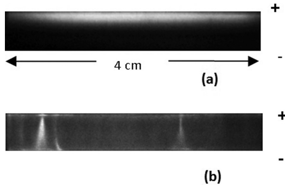
FIG. 4. ICCD images of a DBD in N_2 . (a) Diffuse discharge; (b) Filamentary discharge. Exposure time: 10 ns. 32 Reproduced with permission from Gherardi et al. , Plasma Sources Sci. Technol. 9 , 340 (2000). Copyright 2000 Institute of Physics.
