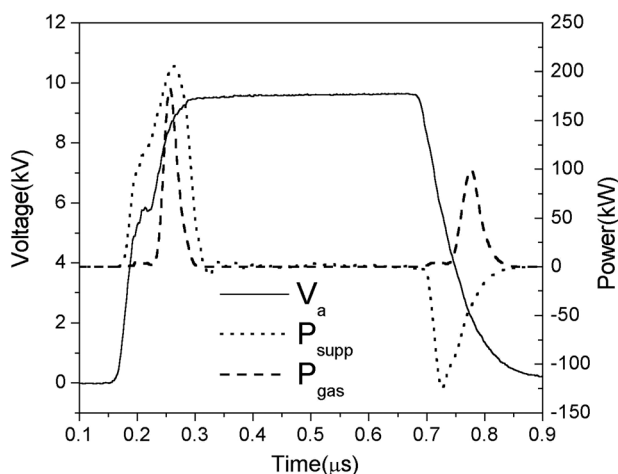
FIG. 12. Applied voltage, supply power, P_{\text{supp}} , and gas dissipated power, P_g , versus time. When P_{\text{supp}} is positive, the power is supplied from the source to load, and when P_{\text{supp}} is negative, the power is restored from the load to source. 24
