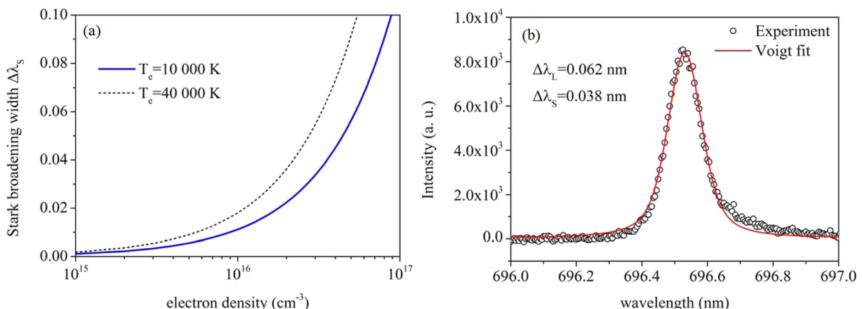
FIG. 20. (a) The relationship between the Stark broadening width and the electron density for T_c = 10\,000 \text{ K} and T_c = 40\,000 \text{ K} . (b) Voigt fitting of the Ar 696.5 nm line profile of the microplasma. 78
