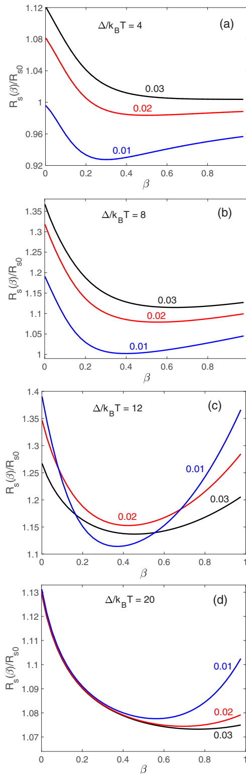
FIG. 11. Minima in R_s(\beta) as a function of the interface barrier parameter \beta calculated at \Delta/k_B T = 4, 8, 12, 20 , \Gamma = 0.01, 0.02, 0.03 , \lambda = 4\xi_S , D_n = 0.1D_s , \alpha = 0.05 , and \hbar\Omega = 11\Delta . Here R_s(T, \beta, \Gamma) are normalized to their respective values R_{s0}(T, \Gamma) for each \Gamma in the absence of the N layer.
