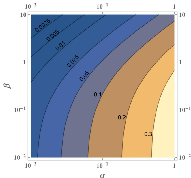
FIG. 3. A contour map of the self-consistent pair potential \Psi calculated from Eq. (43) at k_B T/\Delta = 0.057 and \hbar\Omega = 11\Delta . The parameters \alpha and \beta are defined by Eqs. (11) and (12).
