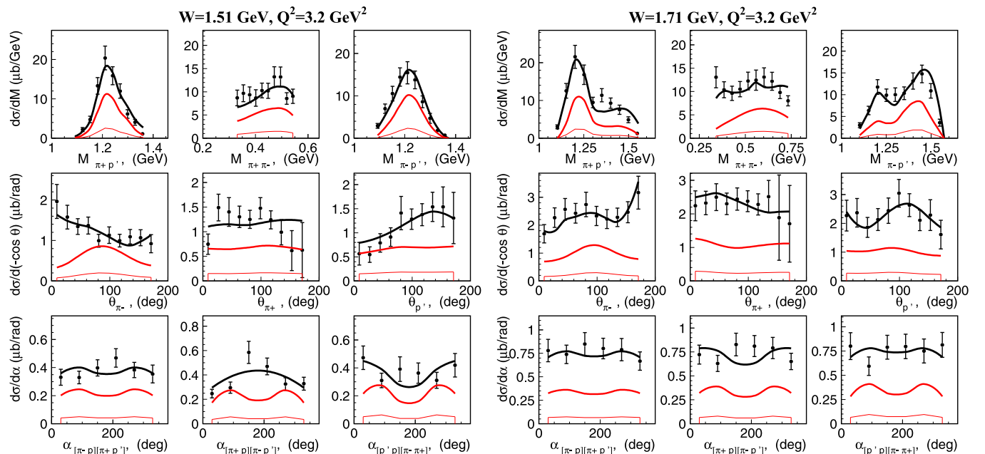
FIG. 19. The resonant contributions from the JM16 model [4,16,18] (red solid lines) to the nine onefold differential \pi^+\pi^-p electroproduction cross sections in representative W bins inside two W intervals of distinctively different resonant content described in Sec. III at Q^2 = 3.2 \text{ GeV}^2 . The model uncertainties for the resonant contributions are shown by the thin red band at the bottom of each plot. The black solid lines represent the full cross sections from the JM16 model.
