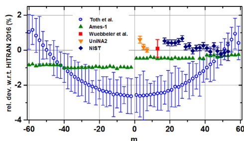
Fig. 7. Comparison of line intensities between HITRAN2016, HITRAN2012 (Toth et al. [88]), and other accurate experimental and theoretical sources for the 20012 - 00001 band (2- \mu m band) of 12 C 16 O 2 : measurements Wuebbeler et al. [102], NIST [104] and UniNA2 [103], and theory Ames-1 [79]. The zero relative deviation line corresponds to HITRAN2016 line intensities (in this case from Zak et al. [82]). The running index m equals -J , J , and J+1 for the P, Q, and R branches, respectively.
