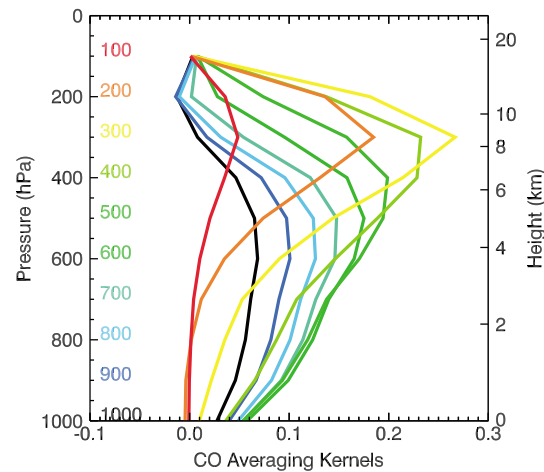
Figure 1. Example of mean averaging kernels for the MOPITT TIR-only product. They correspond to observations acquired on 10 April 2010 between 20°N and 24°N and −160°E and −156° E.
