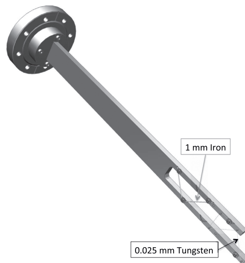
Fig. 3. 2H02A Wire Harp. The wire frame is moved into the beam at 45^\circ .
