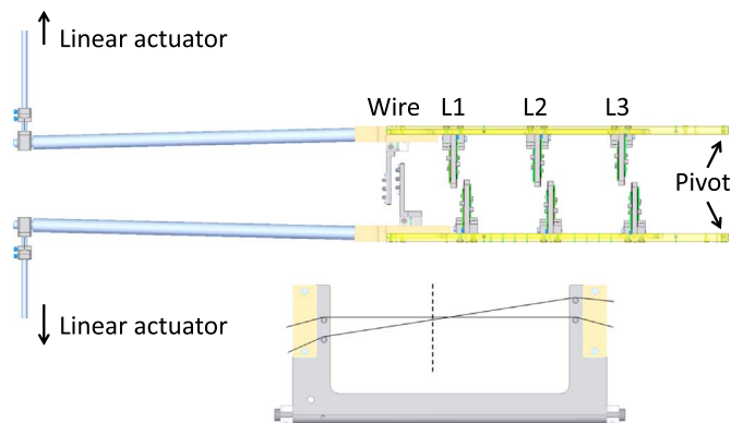
Fig. 4. Elevation view of the SVT motion system and beam’s eye view of the SVT wire scanner with dashed line indicating the nominal horizontal beam position.
