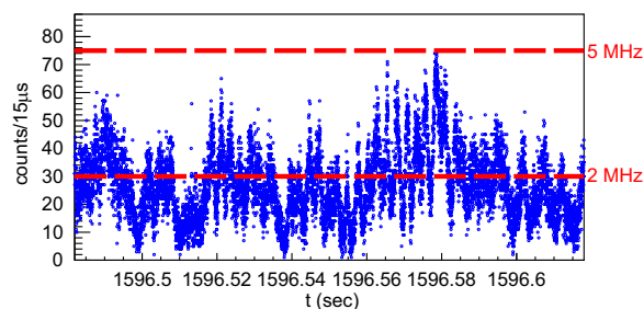
Fig. 9. Oscillations of rates on the halo monitors in the 140 ms time interval.
