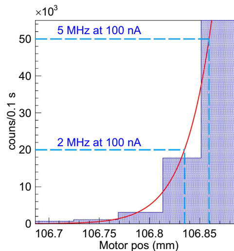
Fig. 10. Counts on the halo monitors as a function of harp motor position. The red solid line is the Gaussian fit to the whole beam profile. The two blue dashed vertical lines show the positions of the wire where rates are 2 MHz and 5 MHz.
