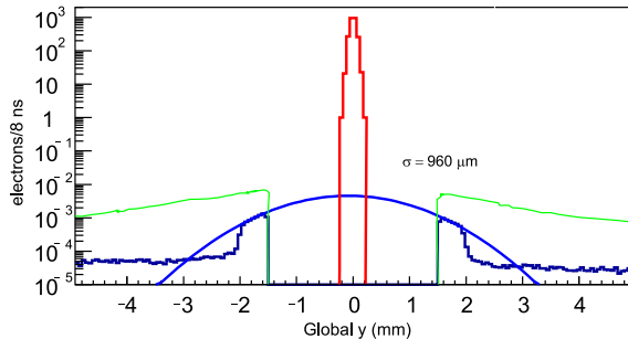
Fig. 12. SVT axial layer 1 occupancy during data taking run (green) and no target run (blue). The histogram in red is nominal 50 nA Gaussian core and the blue curve is a Gaussian fit to the halo with \sigma of 960 \mu m. (For interpretation of the references to color in this figure legend, the reader is referred to the web version of this article.)
