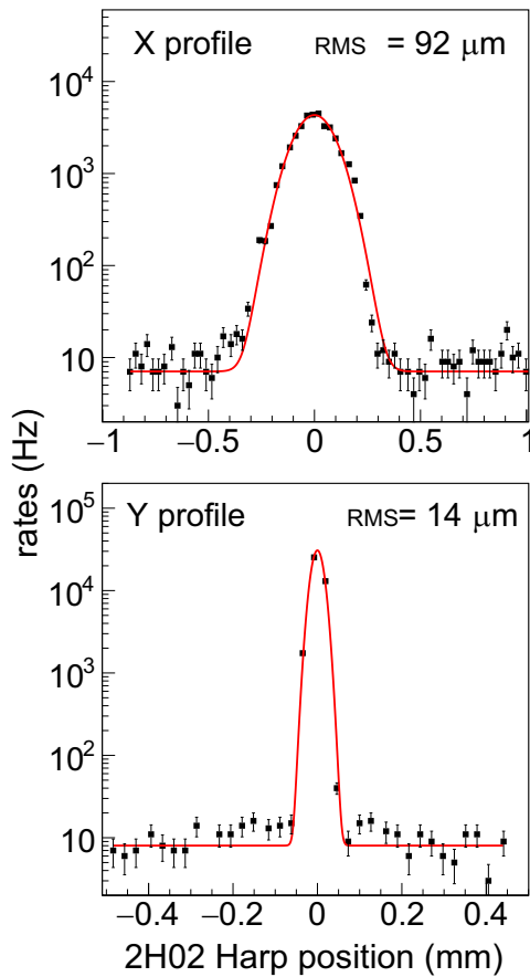
Fig. 6. Beam profile measurement with wire harp 2H02A during the 2.3 GeV run.
