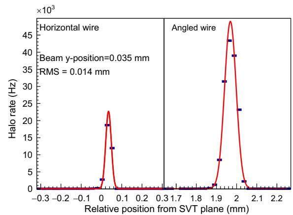
Fig. 8. SVT wire scan.
