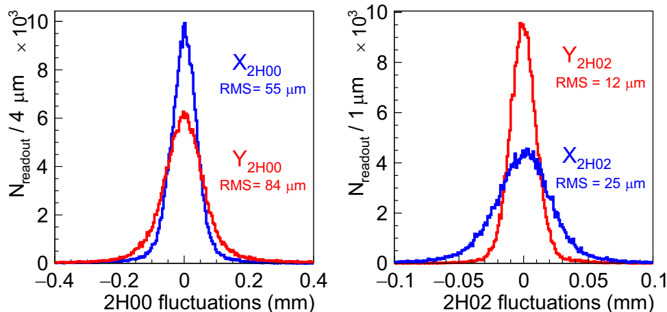
Fig. 7. Distributions of beam positions at BPM 2H00 and 2H02A during the 2.3 GeV run.
