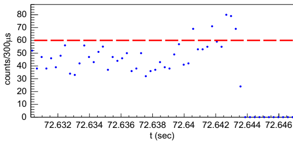
Fig. 11. HPS halo counter rates as a function of time. The FSD integration time is 1 ms and the beam current is 200 nA. Each point represents integrated counts over a 300 \mu s time interval.
