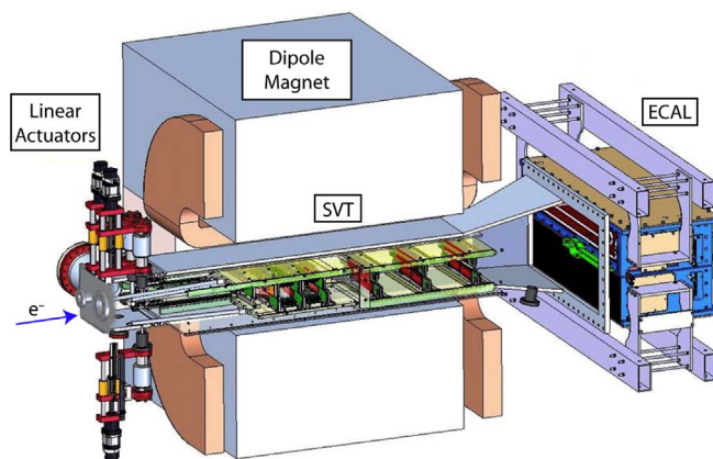
Fig. 2. Partial cut-out view of the HPS setup.
