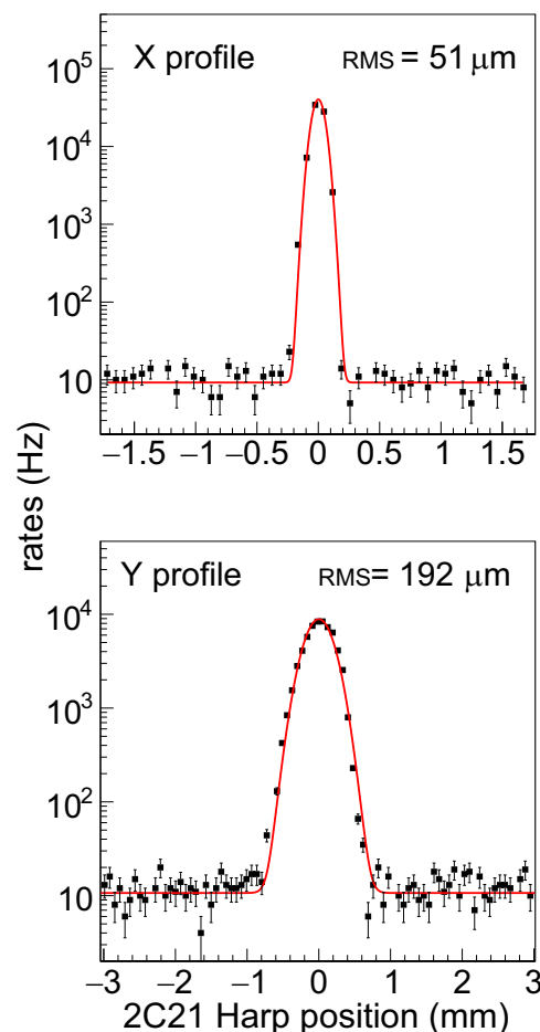
Fig. 5. Beam profile measurement with wire harp 2C21 during the 2.3 GeV run.
