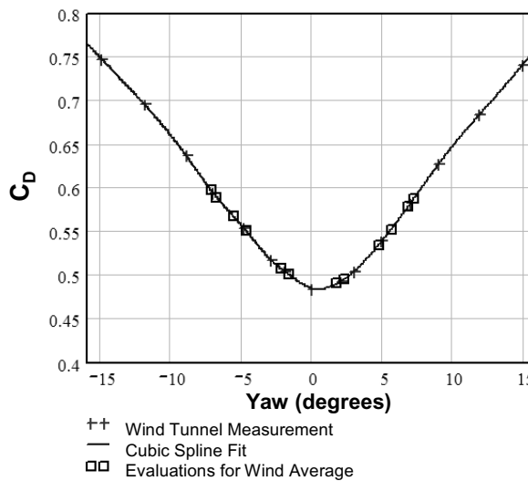
Figure A3 Sample Cubic Spline Fit
