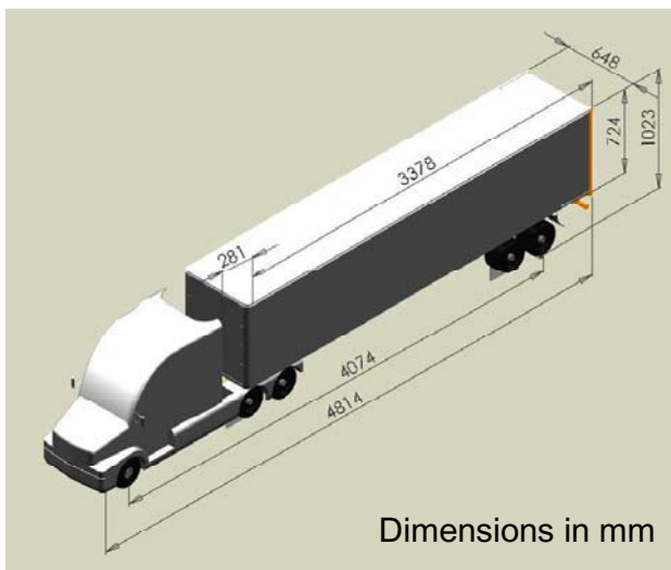
Figure A1 SORHT Model Details
