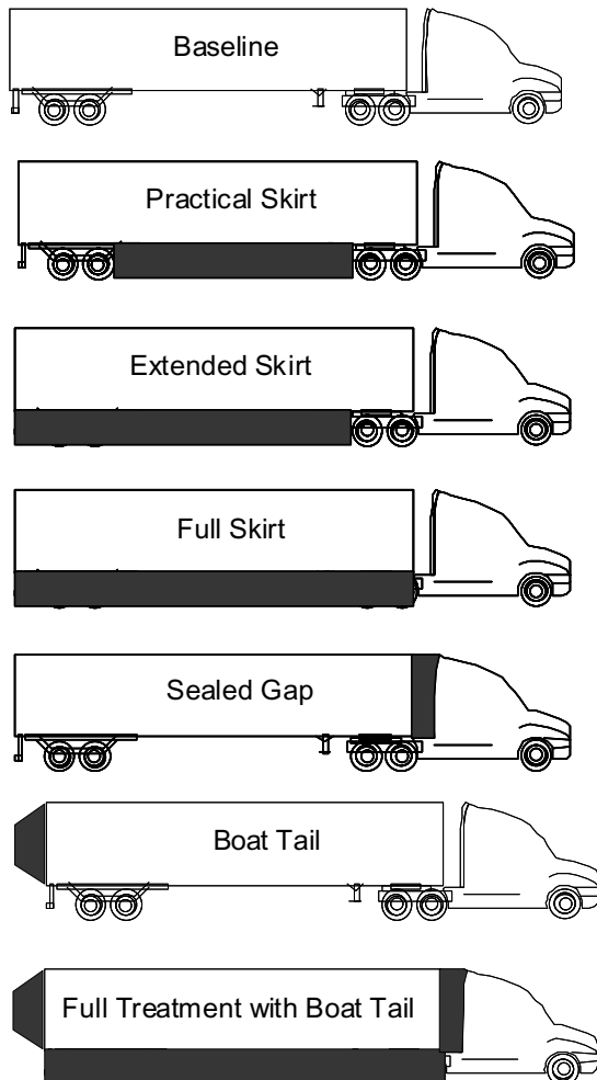
Figure 4 Test Configurations
