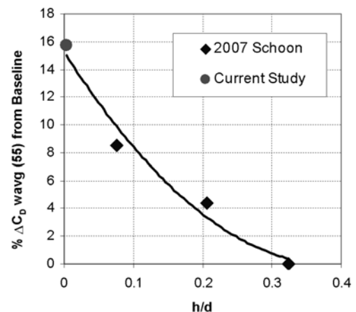
Figure 6 Drag Reduction vs. Non-dimensional Skirt Height
