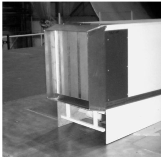
Figure A2 Gap Seal and Boat Tail Treatments
