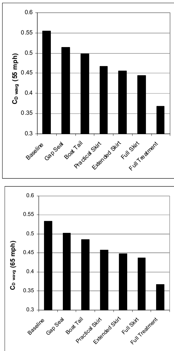
Figure 5 Wind Averaged Drag Coefficients
