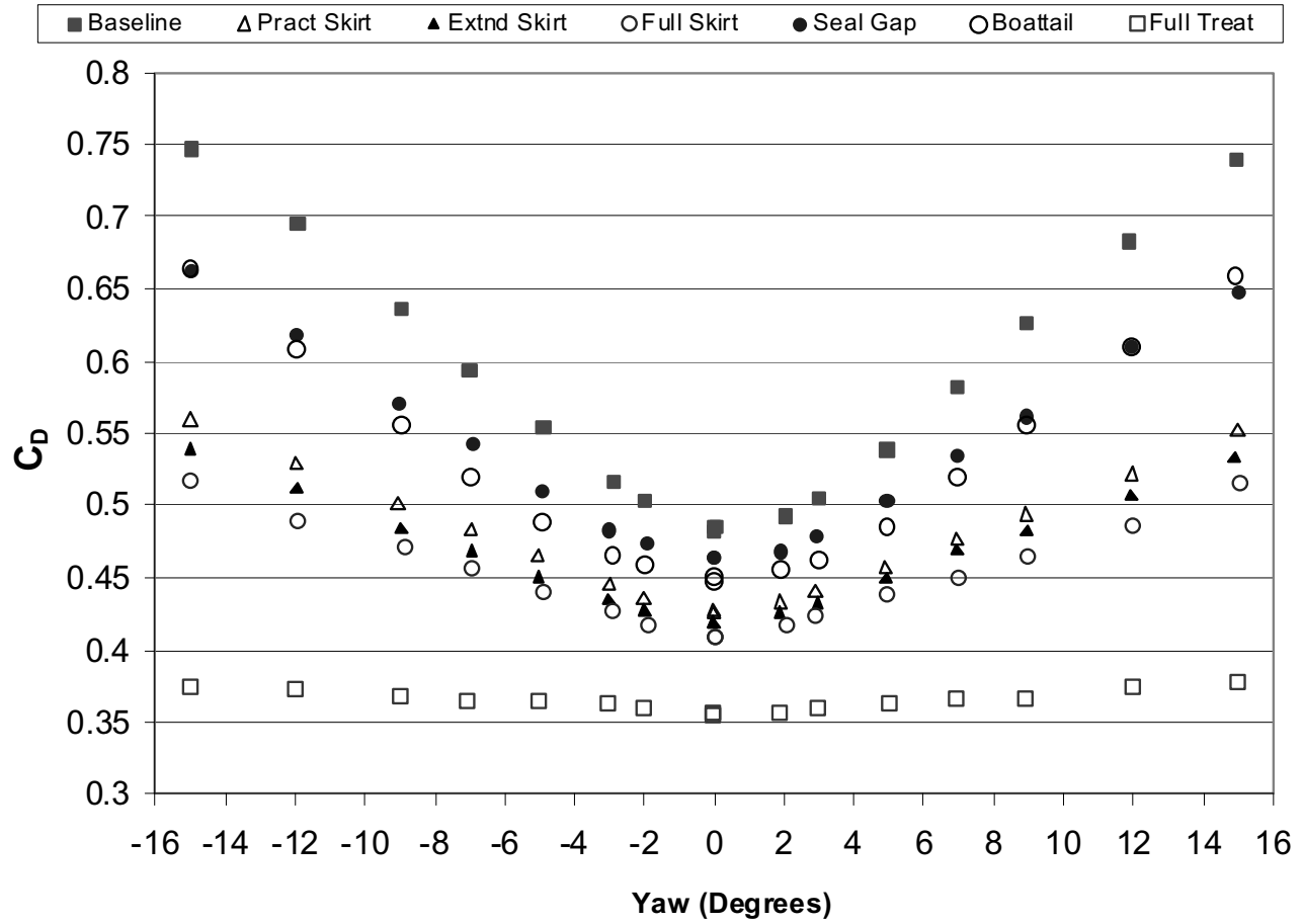
Figure A4 Detailed Configuration Yaw Sweep Data Summary
