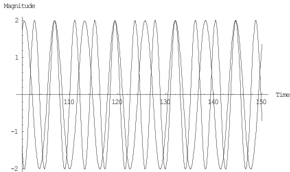
Figure 1. Simulation: two van der pol oscillators, no linkage, no mode-locking (from Selover, Jensen, and Kroll (2003, 2005))
