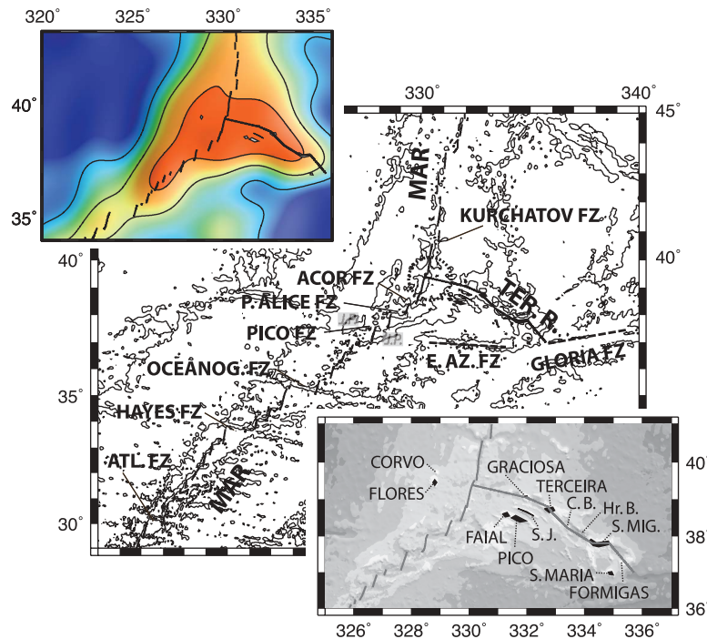
Figure 1. Geological setting of the Azores. Azores TJ is indicated with a dashed circle. MAR = Mid-Atlantic Ridge, TER. R. = Terceira Rift, E. Az. FZ = East Azores FZ, and J.P. = Jussieu Plateau. (Left inset) Filtered bathymetry of the Azores plateau. A lowpass filter with a cutoff wavelength of 300 km was applied to the bathymetry data of Smith and Sandwell [1997]. Contour lines indicate 1.9, 2.7, and 3.5 km depth. (Right inset) Locations of islands in the Azores Archipelago. S.J., S. Mig, C.B., and Hr. B. are Sao Jorge Island, Sao Miguel Island, Castro Bank, and Hirondelle Basin, respectively.
