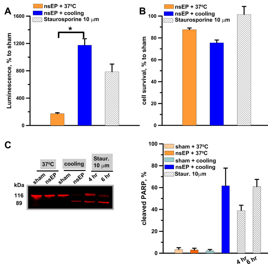
Figure 4. Cooling of nsEP-exposed cells induces caspase 3/7 activation and PARP cleavage. U-937 cells were exposed to 50, 300 ns pulses (100 Hz, 7 kV/cm) and immediately incubated at 37°C, or placed on ice for 30 min and then in the incubator. Panels (A,B) show, respectively, the activity of caspase 3/7 and cell survival at 4.5 hr after nsEP with or without cooling. For a positive control, apoptosis was induced by incubation with 10 μm staurosporine for 4.5 hr. Panel C shows a representative Western blot for intact and cleaved PARP (116 and 89 kDa, respectively) and the quantification of the cleaved fraction at 4.5 hr after nsEP exposure.; For a positive control, apoptosis was induced with 10 μm staurosporine. Mean \pm s.e. n = 6–9 (A,B) or n = 3 (C). * p < 0.001 for the difference of nsEP + cooling from nsEP + 37°C.
