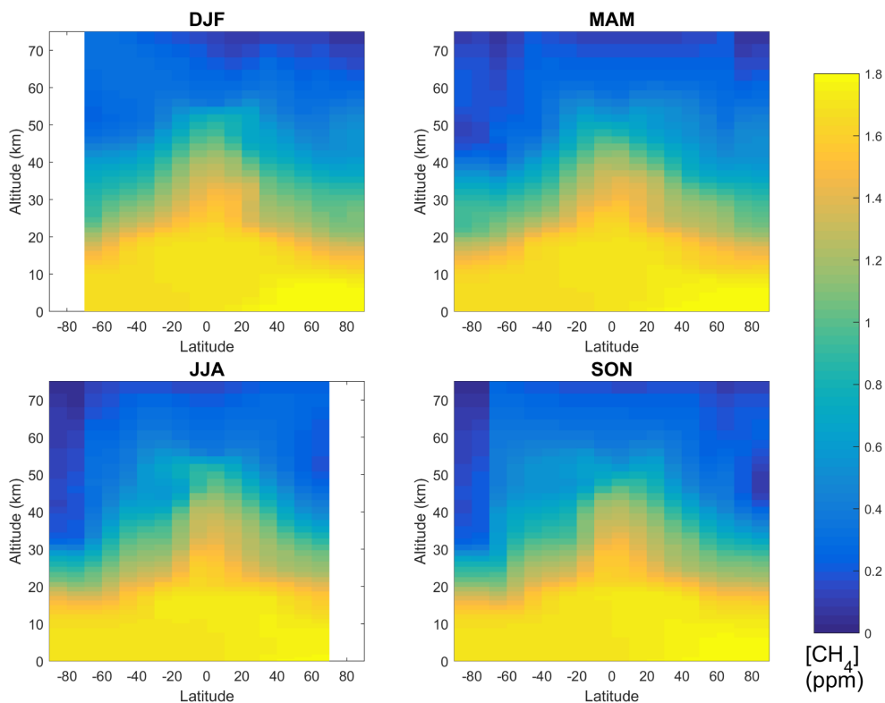
Figure 6. Total methane concentration by season from the ACE-sampled WACCM data set. Especially low levels of CH 4 appear over the South Pole between June and December. In reality, these levels are only present in August and September as shown in the Supplement, but the WACCM sampling method is biased toward those 2 months at those latitudes.
