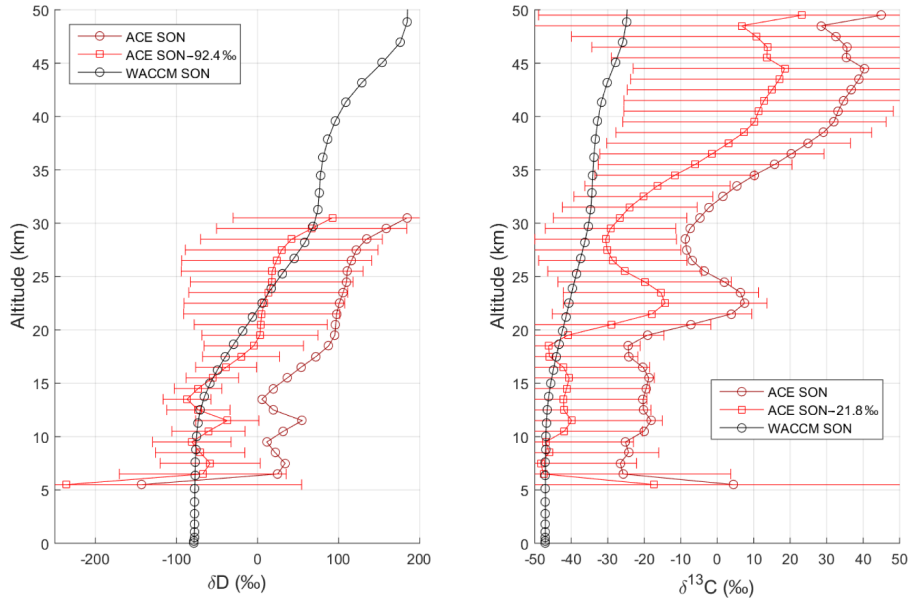
Figure 12. Results of ACE calibration compared to WACCM. Data shown here are from the 60° S September/October/November data bin. The error bars on the calibrated ACE data are equal to 1 standard deviation of the measurements at that altitude.
