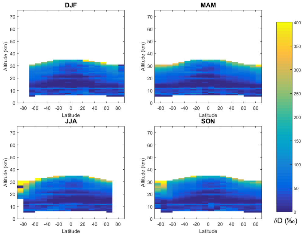
Figure 4. ACE \delta D by season.
