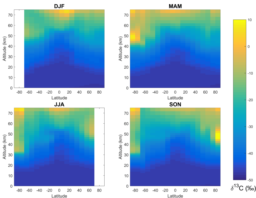
Figure 8. \delta^{13}\text{C} by season from the ACE-sampled WACCM data set.
