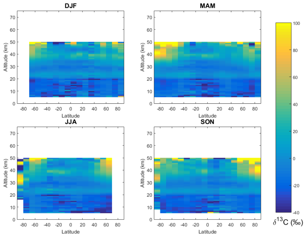
Figure 5. ACE \delta^{13}C by season.
