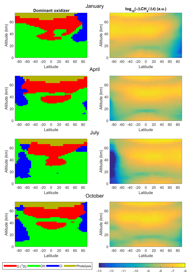
Figure 15. Dominant oxidizing species of \text{CH}_4 by location and season (left) and total methane oxidation (right).
