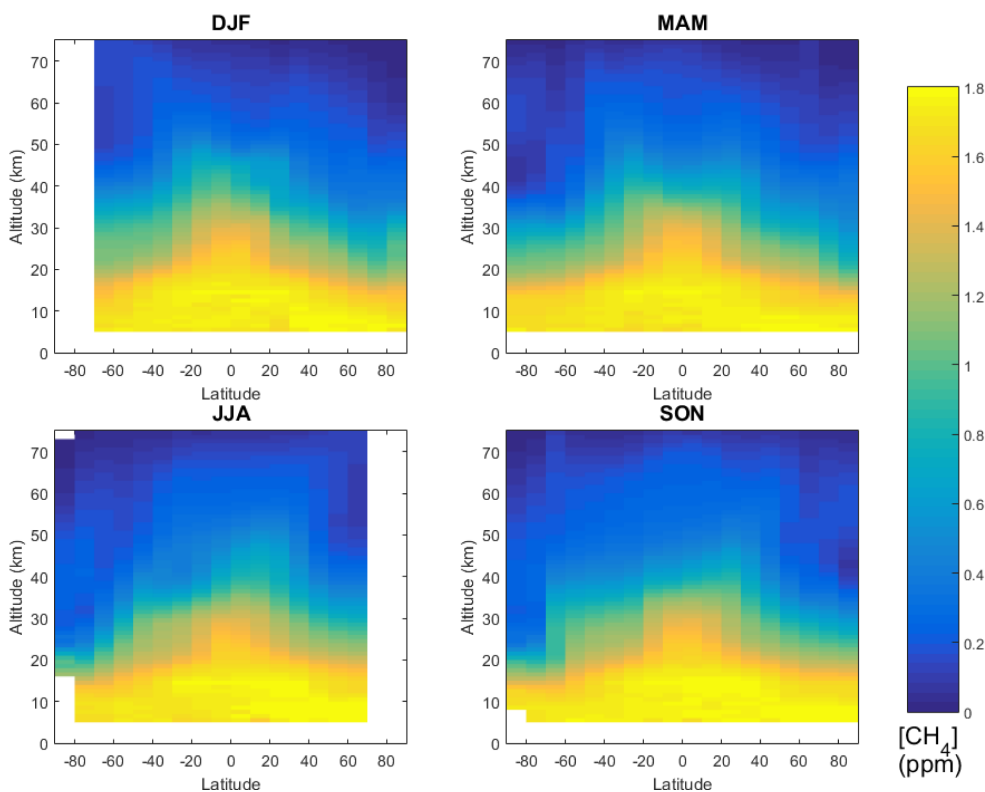
Figure 3. ACE total methane concentration by season.
