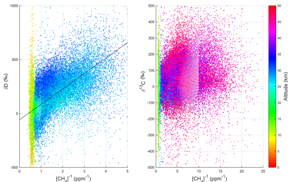
Figure 9. Keeling plots of ACE data for \delta\text{D} (left) and \delta^{13}\text{C} (right). Each data point is color-coded by its measurement altitude. The streaks of data present in the right figure are artifacts; ACE measurements are retrieved to three significant figures, causing a sharp change in precision around 10\text{ ppm}^{-1} (e.g., 9.99\text{ ppm} vs. 10.1\text{ ppm} ).
