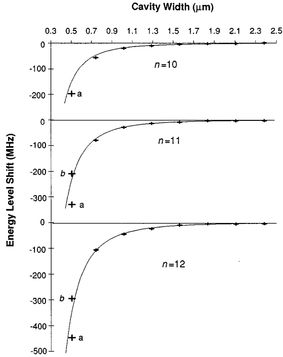
FIG. 4. Measured energy level shifts for 10S , 11S , and 12S states as a function of cavity width. Labels a and b mark two different runs at 504-nm cavity width. Data for larger cavity widths are reproduced from our earlier publication [1]. Solid curves are theoretical predictions of the Lennard-Jones theory for an atom at the center of a parallel-plate cavity.
