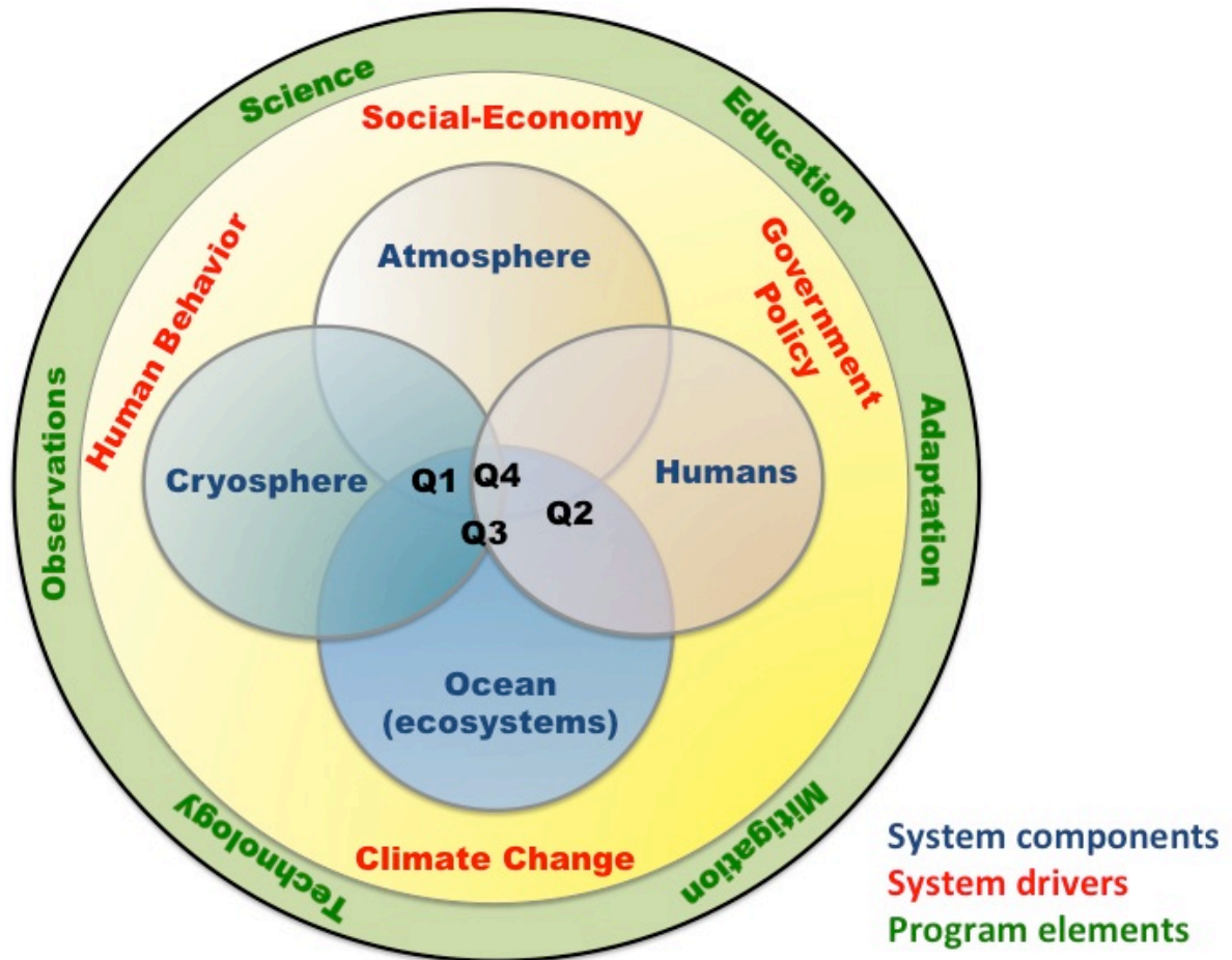
Figure 2. Diagram illustrating components of the North Atlantic-Arctic system, including system interactions (overlapping circles) and drivers (red), as well as key elements of an international multidisciplinary North Atlantic-Arctic program. The overarching research Questions 1-4 (Q1-4) presented in the science plan include aspects of all the system components and their placement on the diagram indicates the key systems involved.
