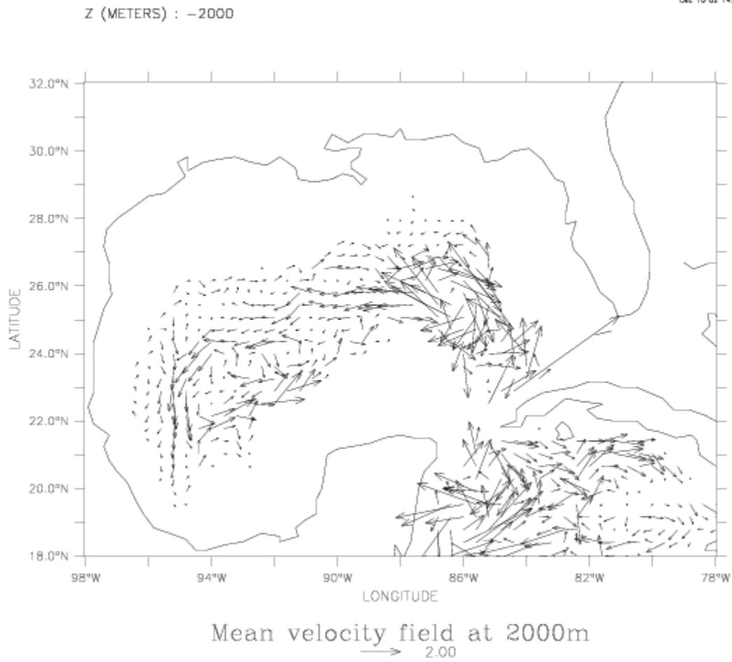
Figure 5.5. The mean velocity field from the MICOM model at a depth of 2000 m.
