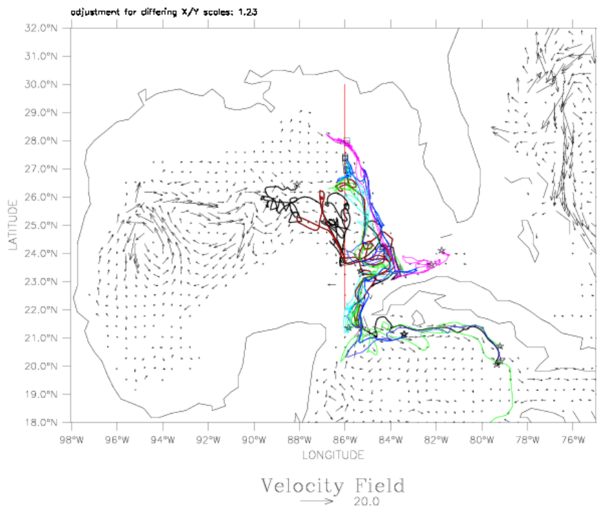
Figure 5.11. The Lagrangian trajectories of particles in layer 13, originating in the northern and central regions of the Gulf. The particles are launched along the red N-S line at the squares; the end points of the paths are shown by the stars.
