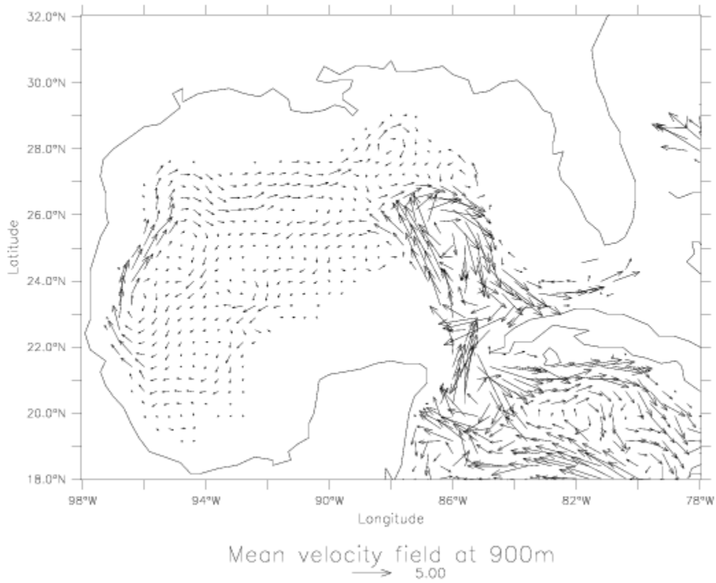
Figure 5.2 The mean velocity field from the MICOM model at a depth of 900m.
