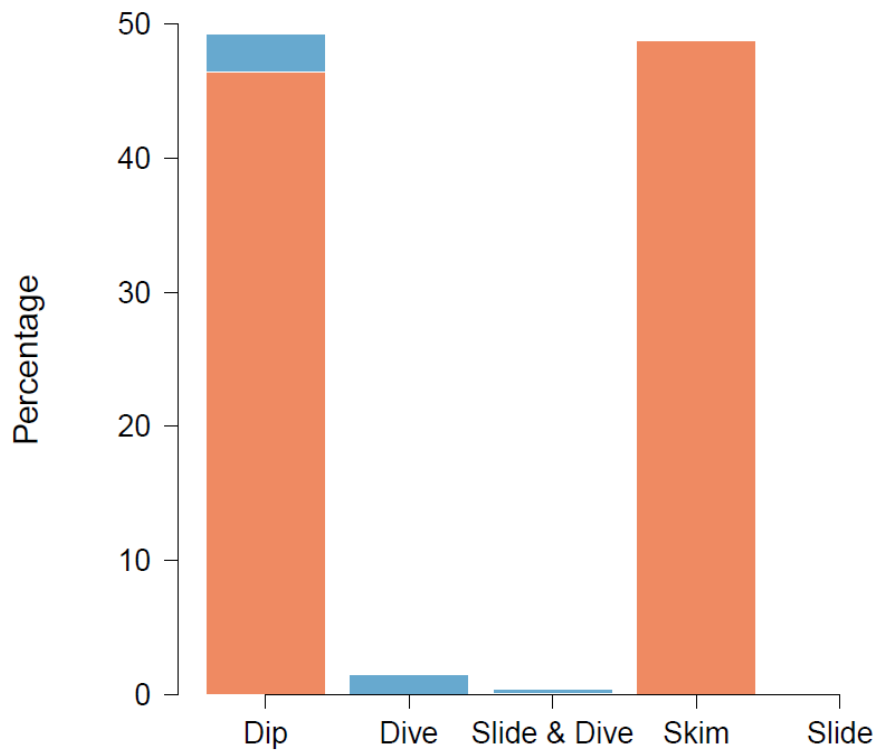
Robots (34,203 sessions)
