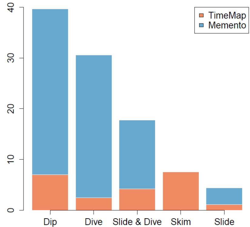
Humans (3,431 sessions)
