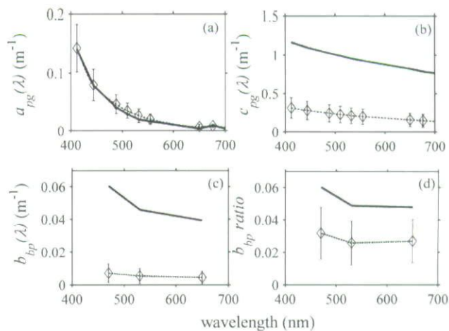
Fig. 3. Inherent optical properties measured at the whittings station (solid line) compared to the mean (dot-dashed line) and standard deviation (errorbars) measured at twenty-one other stations located throughout the Bahama Banks: (a) absorption by particulate and dissolved material ( a_{pg} ); (b) attenuation by particulate and dissolved material ( c_{pg} ); (c) backscattering of particulate; and (d) backscattering ratio illustrating high mineral content at the whittings station.
