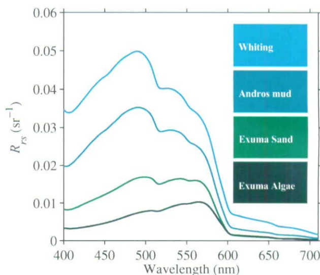
Fig. 6. Remote sensing reflectance, R_{rs} , measured over a selection of stations with 5 m depth and benthic constituents varying from whittings station, Andros mud, Exuma sand, and Exumas algal-covered grapestone sediment. Line colour and coloured boxes show the perceived colour of each spectrum quantified following the approach in Dierssen et al. (2006).
