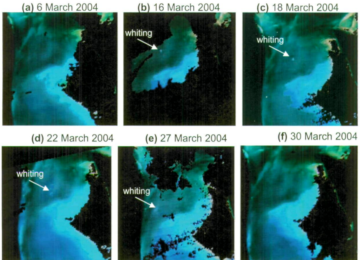
Fig. 7. Pseudo true colour images from the MODIS Aqua satellite obtained on clear sky conditions during the March 2004 field campaign. Patches of turbid white water have been identified visually in several of the images.
