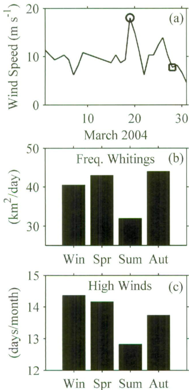
Fig. 9. (a) Maximum sustained wind speed ( \text{m s}^{-1} ) from the Nassau meteorological station for the month of March 2004 highlighting wind speed during the whiting event. (b) Seasonal frequency index of whittings determined on the Great Bahama Bank from low earth orbit space shuttle photography obtained sporadically from 1965–1993 (adapted from Robbins et al., 1997). (c) Seasonal frequency (number of days per month) of maximum sustained wind speeds at the Nassau meteorological station exceeding 7.35 \text{ m s}^{-1} , which is the threshold estimated to cause 5-m penetrating Langmuir cells in waters with low stratification (buoyancy frequency of 0.02 \text{ s}^{-1} ).
