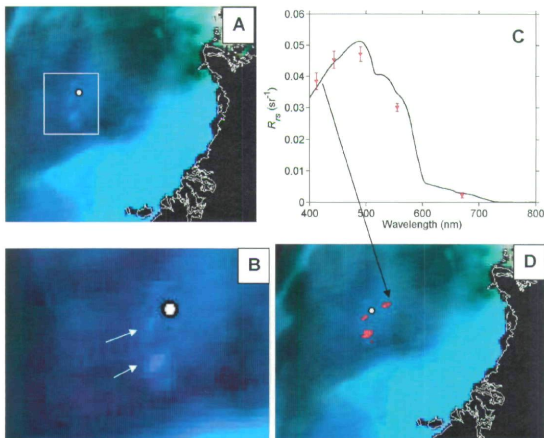
Fig. 8. (a) MODIS pseudo true colour image from 27 March 2004 showing the location of the whittings station (white circle) and Andros Island outlined to the east. The whiting was encountered in the field one day later on 28 March 2004. (b) Highlight of region from (a) with arrows pointed to the highly reflective regions; (c) Spectral remote sensing reflectance, R_{rs} , from the whittings patches in the atmospherically-corrected MODIS imagery (red points with error bars) compared to in situ R_{rs} measured at the whittings station (black line). (d) Red regions identified as having spectral R_{rs} closely corresponding to the in situ whittings R_{rs} .
