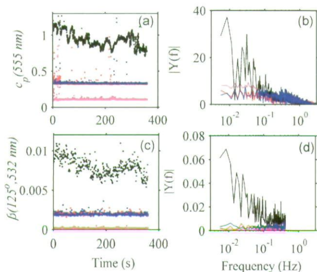
Fig. 4. (a) Time series of particulate attenuation, c_p(555) , measured at the whittings station (#19, black), compared to other stations in the vicinity (#18, 21, blue and red) and the Exumas station (#7, magenta). (b) Fourier transform of the data from (a). (c) Time series of the 1.2 Hz backscattering data from the ECO-VSF, \beta_{125^\circ, 532 \text{ nm}} ; (d) Fourier transform of data from (c).
