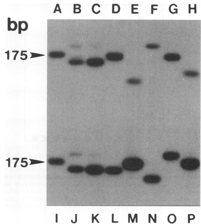
FIG. 3. 16S rDNA fingerprinting of RFLPs from clones representing OTUs with oligonucleotide probe 536F. Lanes A, I, and P, OTU 1 clones; lanes B and J, OTU 2 clones; lanes C and K, OTU 3 clones; lane D, OTU 4 clone; lane E, OTU 5 clone; lane F, OTU 6 clone; lane G, OTU 7 clone; lane H, OTU 8 clone; lane L, OTU 9 clone; lane M, OTU 10 clone; lane N, OTU 11 clone; lane O, OTU 12 clone. Two or three lanes containing members of the same OTU demonstrate that there was reproducibility among different 16S rDNA clones in that OTU.
