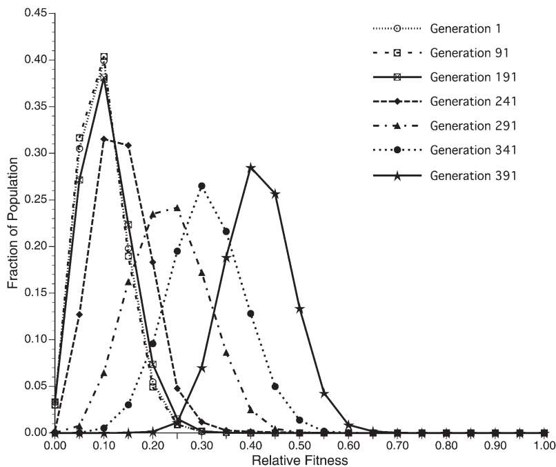
Figure 6. The frequency of adult fitness over a suite of selected generations for the Delaware Bay base case. In this simulation, Dermo disease entered the population at generation 201 with a disease intensity set at level 3 (Fig. 8). The trajectory for adult fitness improvement is shown in Figure 9. The distribution of adult fitness values for the naïve population is shown for generations 1, 91, and 191. During this time, alleles conferring disease resistance were allowed to drift without selective advantage for 200 generations. The resulting frequency shifts by drift only modestly in comparison with generations greater than 200.
