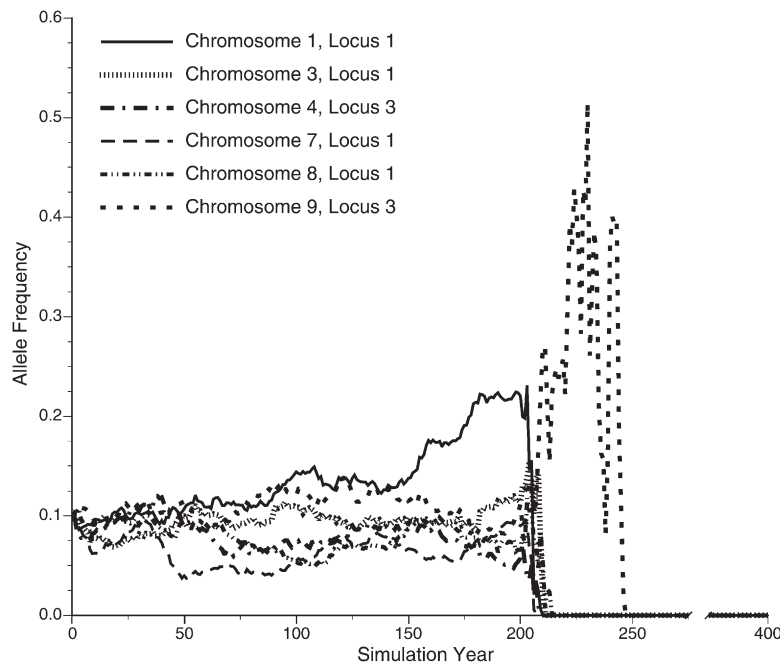
Figure 10. Trajectories of allelic frequencies for alleles conferring disease resistance that were lost through drift in the Delaware Bay case with high disease pressure (level 4). Exposure to disease in the naïve population commenced in generation 201. The depicted alleles were lost between generations 201 and 250.
