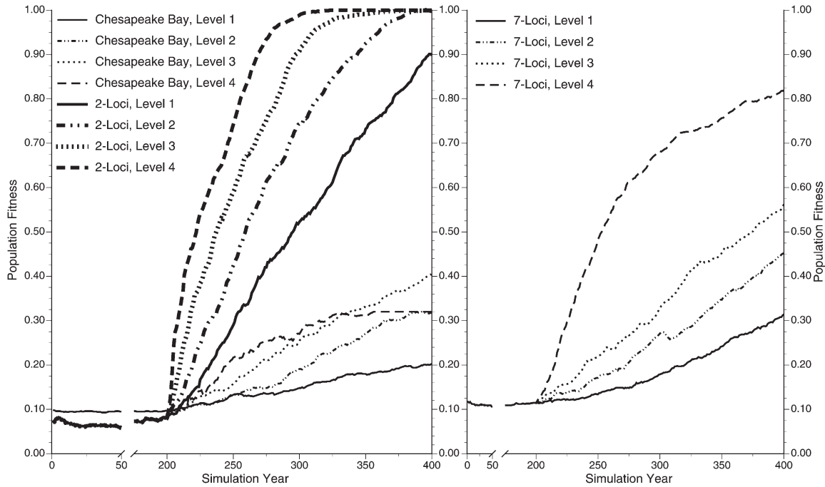
Figure 14. Comparison between population fitness for 4 disease pressures for oysters parameterized for Chesapeake Bay with 2 (2-Loci), 7 (7-Loci), or 14 (Chesapeake Bay) loci contributing to disease resistance (Table 2). The naïve, unexposed case is shown for generations 0–200. Population fitness ranges from 0–1.
