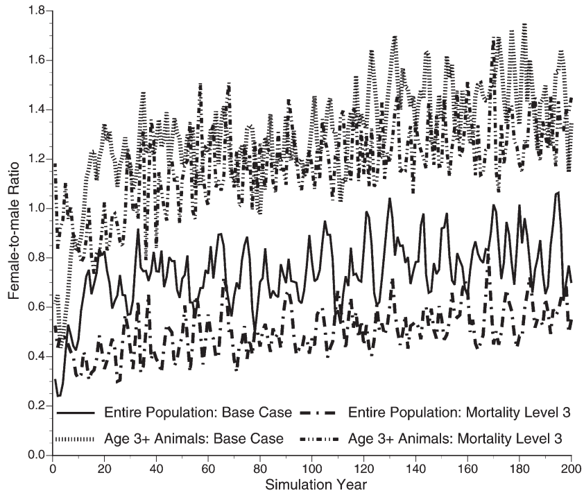
Figure 5. Female-to-male ratio for the entire population and for animals 3 y or more of age for the Delaware Bay base case and for a case influenced by an increment of mortality to level 3 (about 25% per year).
