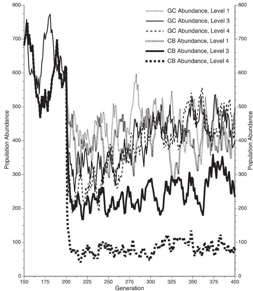
Figure 11. Comparison between population abundance in populations exposed to 3 disease pressures for oysters parameterized for Chesapeake Bay (CB) and the Gulf coast (GC; Table 2). The naïve, unexposed case is shown for generations 150–200. The 3 levels of disease exposure begin in generation 201. Population fitness trajectories are shown in Figure 9.
