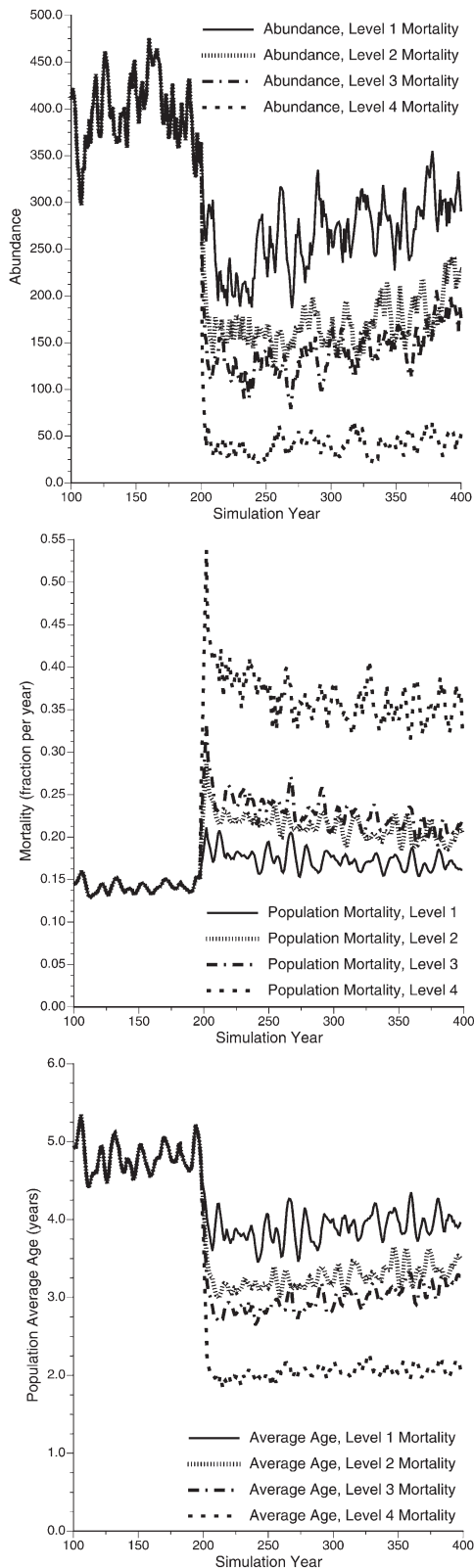
Figure 7. Comparison of population abundance (top), population mortality rate (middle), and population average age (bottom) after the onset of disease at generation 201 for the 4 degrees of pathogen virulence and commensurate increases in natural mortality rate. Abundance and average age slowly increase over the last 200 generations in some cases because the population develops a degree of disease resistance and, thus, survival increases.
