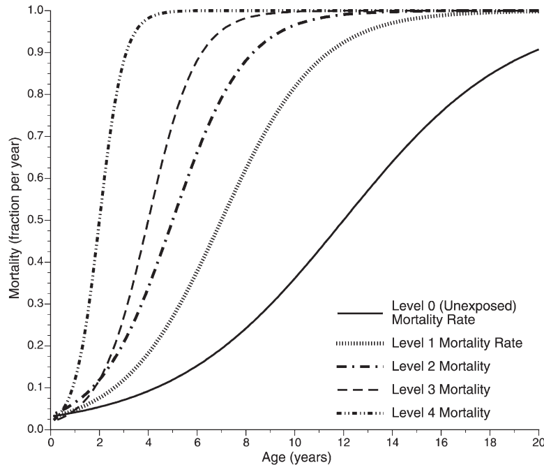
Figure 8. The range of age-dependent mortality rates used in simulations described in Table 2. Level 0 represents the predisease mortality rate for oyster populations in the Mid-Atlantic region. Levels 2 and 3 are consistent with whole-stock Dermo mortality rates observed in Delaware Bay, as well as the mortality rate observed on the medium-mortality beds in Delaware Bay and for the third epizootic on the high-mortality beds of Delaware Bay. Level 4 is a representative mortality rate for the Gulf of Mexico and for the 2 initial epizootics in the high-mortality region of Delaware Bay. Bed allocation to bed groups is defined in Powell et al. (2008) (see also Fig. 15).
