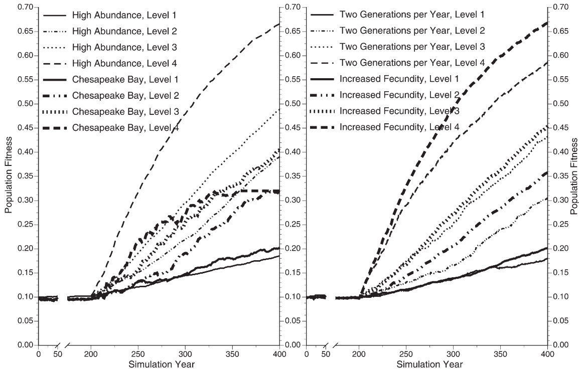
Figure 13. Comparison between population fitness for 4 disease pressures for oysters parameterized for Chesapeake Bay, but with increased population abundance generated by increased carrying capacity (High Abundance) and increased fecundity produced by an increase in the number of successful mating pairs (Increased Fecundity), relative to Chesapeake Bay without these effects (Table 2). Also included is the case of a Gulf of Mexico population with 2 generations per year. The naïve, unexposed case is shown for simulation years 0–200. The 4 levels of disease exposure begin in year 201. Population fitness ranges from 0–1. Note that the y-axis scale only reaches 0.7.
