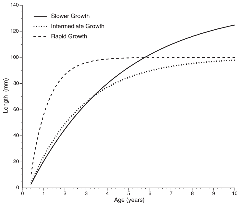
Figure 1. The 3 von Bertalanffy curves used. The rapid-growth curve is from Addison (2006) for oysters from Hackberry Bay and Snail Bay, LA. The intermediate-growth and slow-growth curves come from Chesapeake Bay and Delaware Bay populations, respectively.
