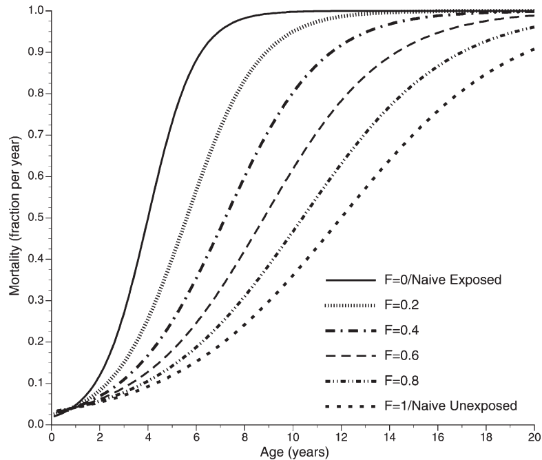
Figure 2. An example of the mortality trends with age for adult fitness varying by 0.2 units from a minimal value of 0 to a maximal value of 1. The adult-fitness-of-0 case ( F = 0 , or naïve exposed) yields a population mortality rate of about 25% for this parameterization of Eqs 8 and 9. The adult-fitness-of-1 case ( F = 1 , or naïve unexposed) yields a population mortality rate of about 13%.
