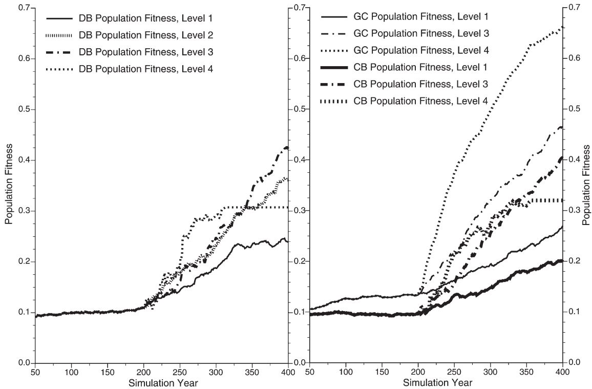
Figure 9. Population fitnesses for the Delaware Bay case (DB), the Chesapeake Bay case (CB), and the Gulf coast (GC) for various levels of initial pathogen virulence and commensurate population mortality (Table 2). The naïve, unexposed case is shown for generations 50–200. The 4 levels of disease pressure begin in generation 201. Fitness ranges from 0–1. Note that the y-axis scale reaches only 0.7.
