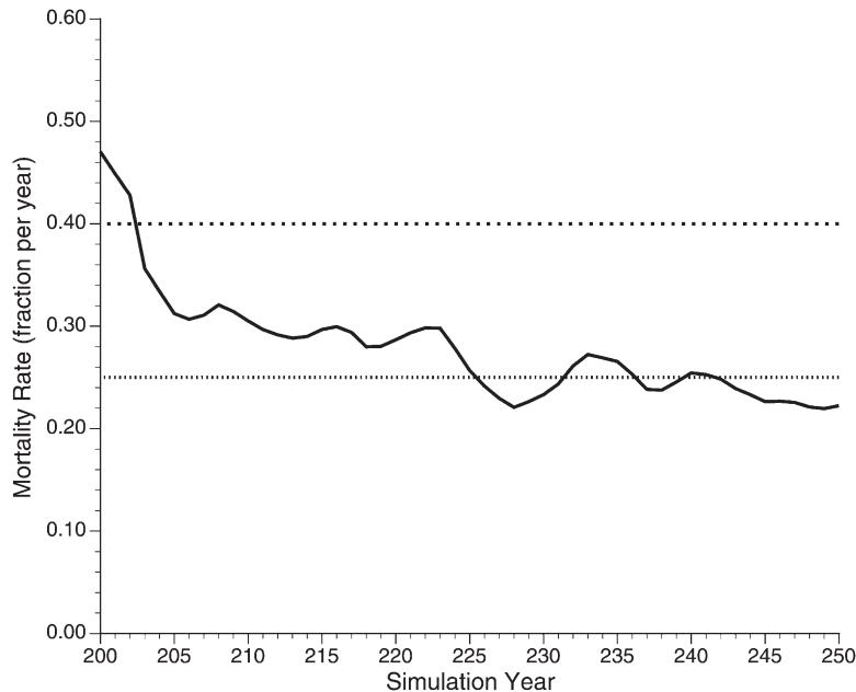
Figure 17. Trends in population mortality rate for the case of high disease pressure (level 4) and a high population abundance (Table 2, Fig. 13) for the 50-y period immediately after the onset of disease. Dotted lines record the approximate mortality rate at disease onset for disease pressures at level 4 (0.4) and level 3 (0.25).
