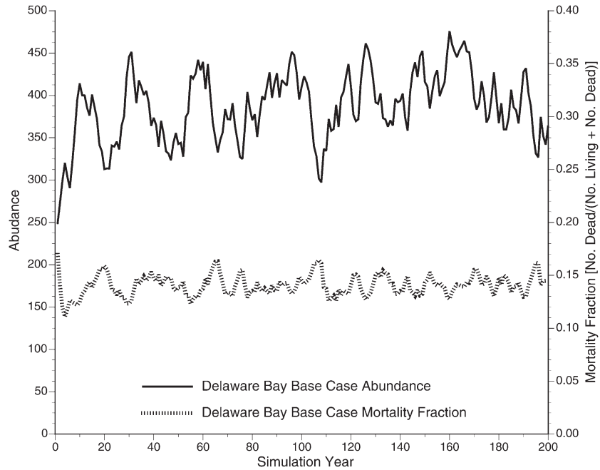
Figure 3. The time series of abundance and mortality rate, represented as the fraction dying each year, for the Delaware Bay base case (Table 2).
