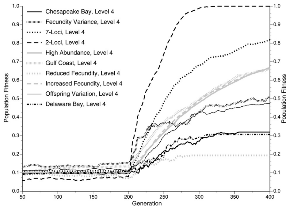
Figure 19. Comparison between a range of cases in which Dermo disease reached epizootic mortality rates of about 40% per year at its onset in generation 201. Legend titles refer back to earlier figures (Figs. 9, 12, 13, and 14).
