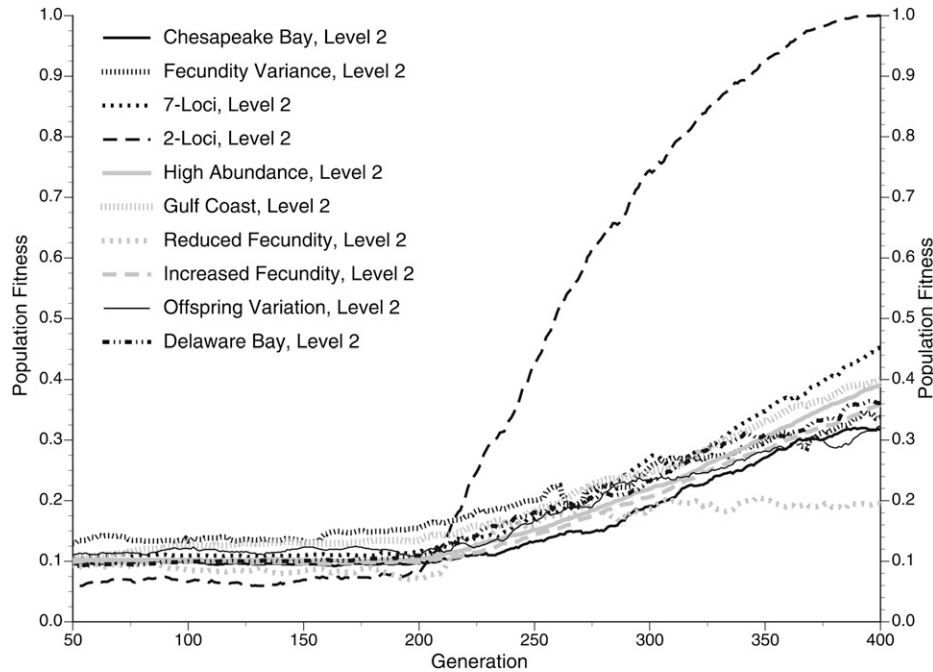
Figure 18. Comparison between a range of cases in which Dermo disease reached epizootic mortality rates of about 22% per year at its onset in generation 201. Legend titles refer back to earlier figures (Figs. 9, 12, 13, and 14).
