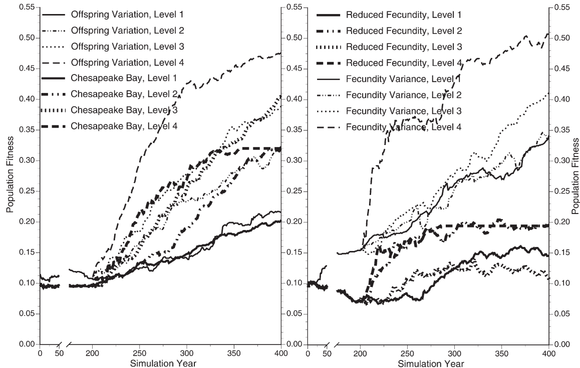
Figure 12. Comparison between population fitness for 4 disease pressures for oysters parameterized for Chesapeake Bay with variation in the number of offspring produced per mating pair (Offspring Variation) with a variable proportion of the population mating (Fecundity Variance), and with reduced fecundity resulting from smaller effective population size (Reduced Fecundity) relative to the Chesapeake Bay case without these effects (Table 2). The naïve, unexposed case is shown for generations 1–200. The 4 levels of disease exposure begin in generation 201. Population fitness ranges from 0–1. Note that the y-axis scale only reaches 0.55.
