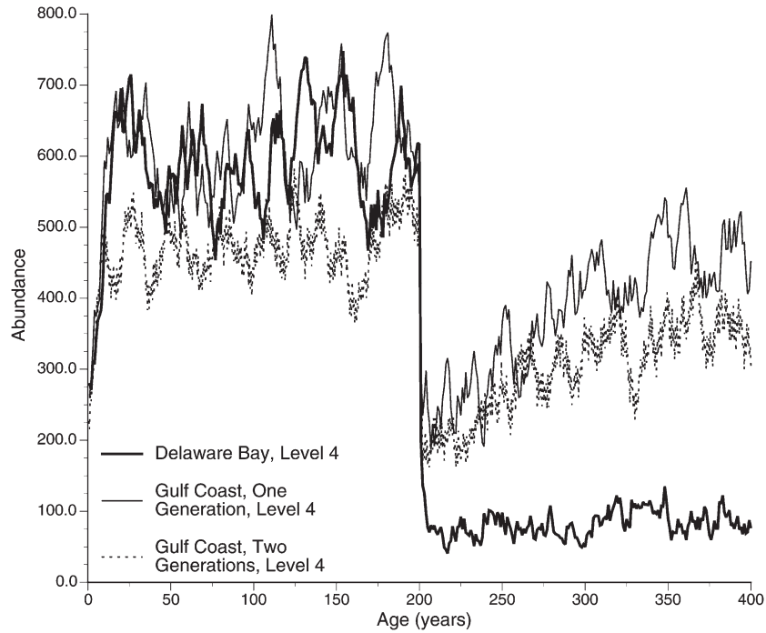
Figure 16. Comparison between population abundance after onset of Dermo disease in year 201 for slow (Delaware Bay) and fast (Gulf Coast) growth rates and for the Gulf coast case with 2, rather than 1, generations per year.
