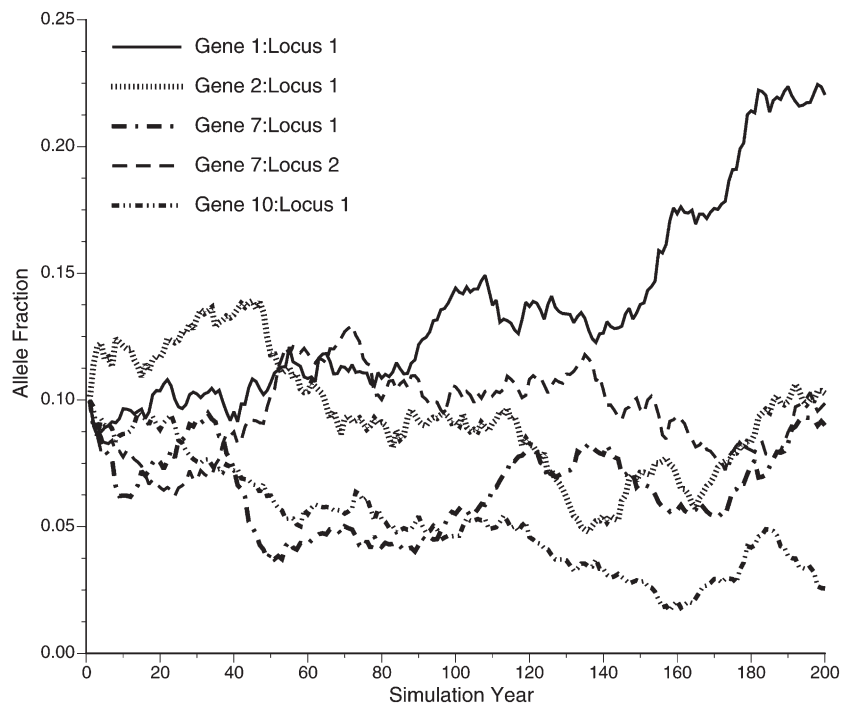
Figure 4. Trajectories for 5 representative alleles conferring disease resistance for the Delaware Bay base case (Table 2). Dermo disease was not present; thus, these alleles drifted over time as neutral alleles. Initial allelic frequency was near 10%.
