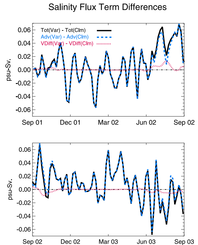
Figure 11. Difference in salinity flux balance terms between the VARICE and CLMICE simulations for the volume below 200 m in the area defined by the HSSW box in Figure 3. Note that one pass of a 1-2-1 smoother has been applied to each difference term.
