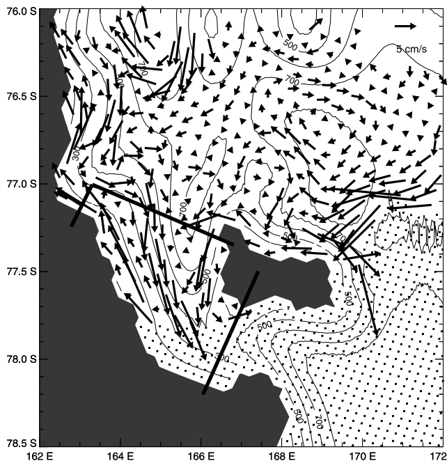
Figure 12. Model circulation at 20 m averaged over January and February for both years for the CLMICE case. The box represents the area over which the averages in Figures 15 and 16 are calculated. Black areas are land masked points and dotted areas represent ice shelf covered water points.
