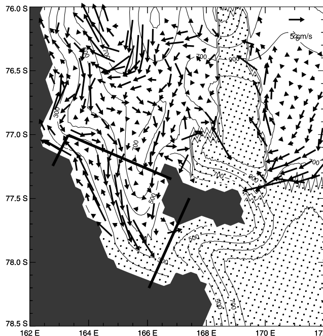
Figure 13. Model circulation at 20 m averaged over January and February for both years for the ICEBERG case.
