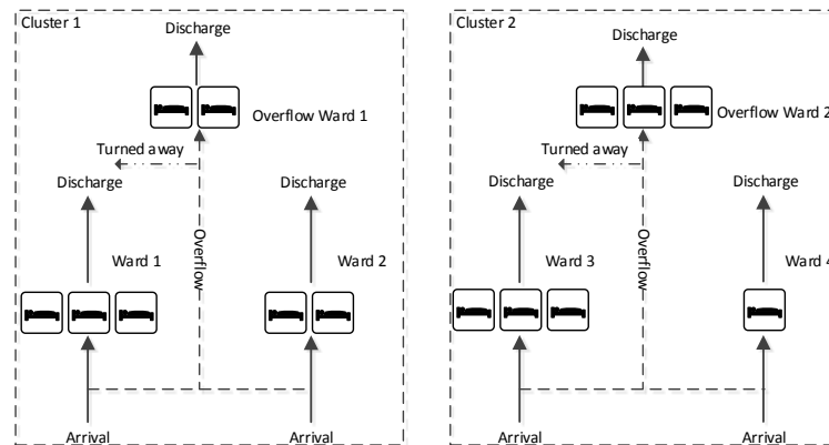
Figure 1 A Clustered Overflow Configuration with 14 Beds, 4 Specialties and 2 Clusters; Cluster 1 (2) Includes Specialties 1 and 2 (3 and 4).
