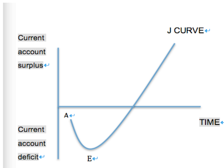
Figure 4.2, The J-curve Effect
