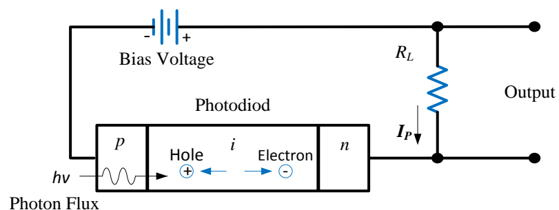
Figure 2.11: PIN photodetector schematic diagram [44], [46].
