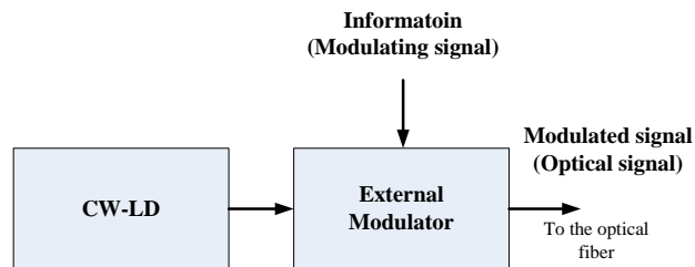
Figure 4.20. External modulator diagram
