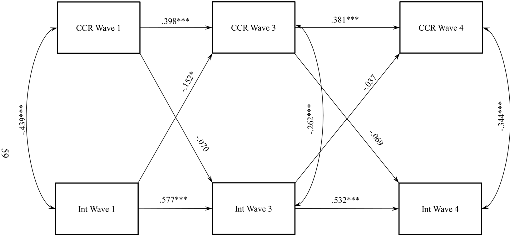
Figure 3: Autoregressive Cross-Lagged Model of CCR and Youth Internalizing Symptoms
