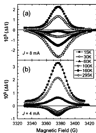
Fig. 1. The positive spin 1/2 PLDMR in Alq_3 thin films. 3
