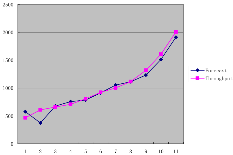
Figure 4 - Fitting graph of exponential smooth
