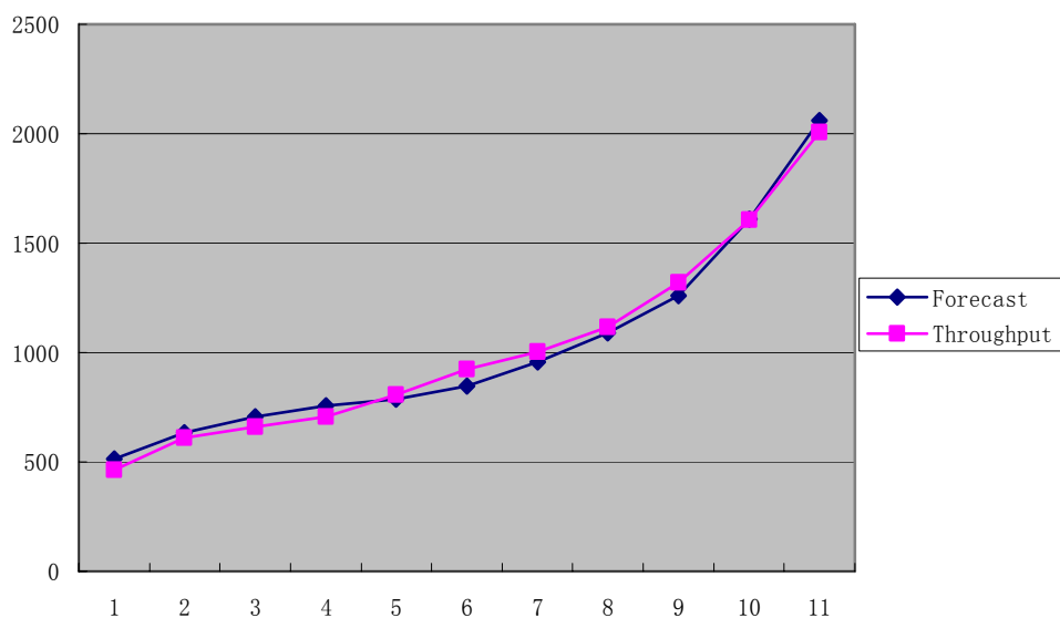
Figure 3 - Fitting graph of regression
