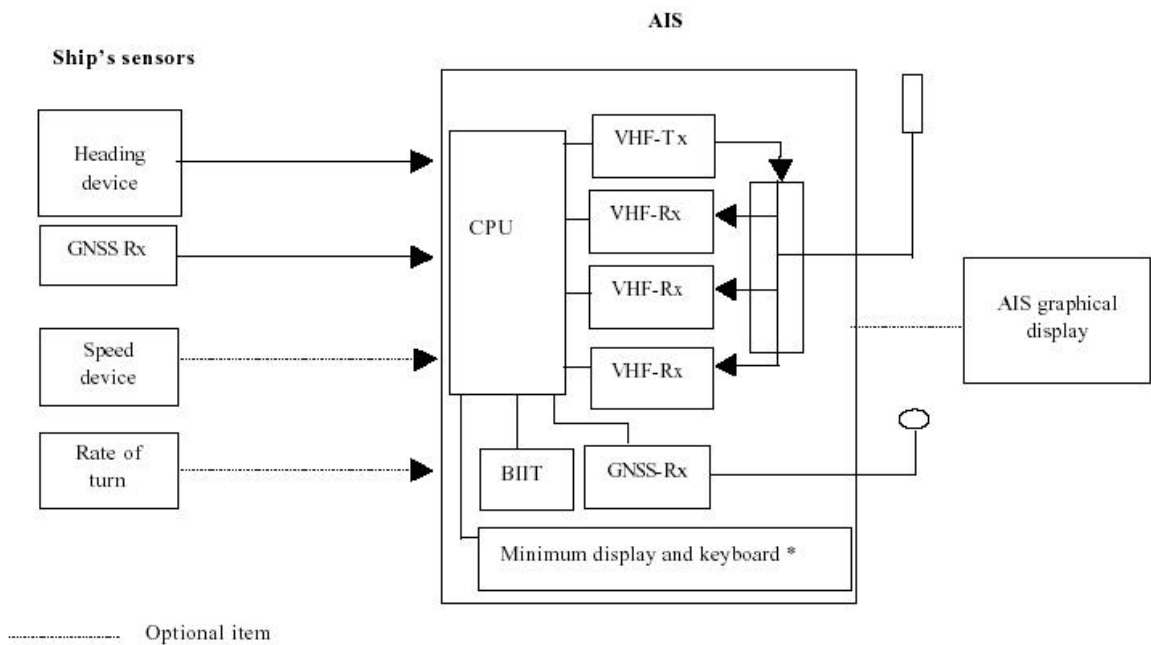
Figure 2 - AIS Components
