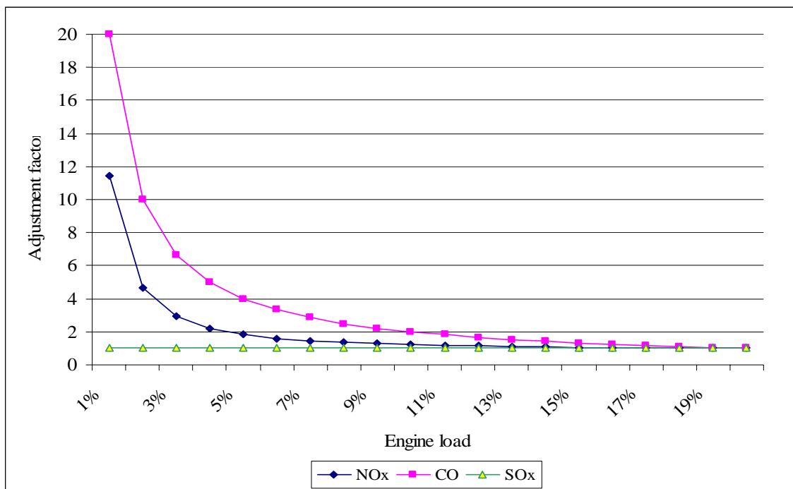
Figure 13 The emission factor adjustment values at low loads below 20%
