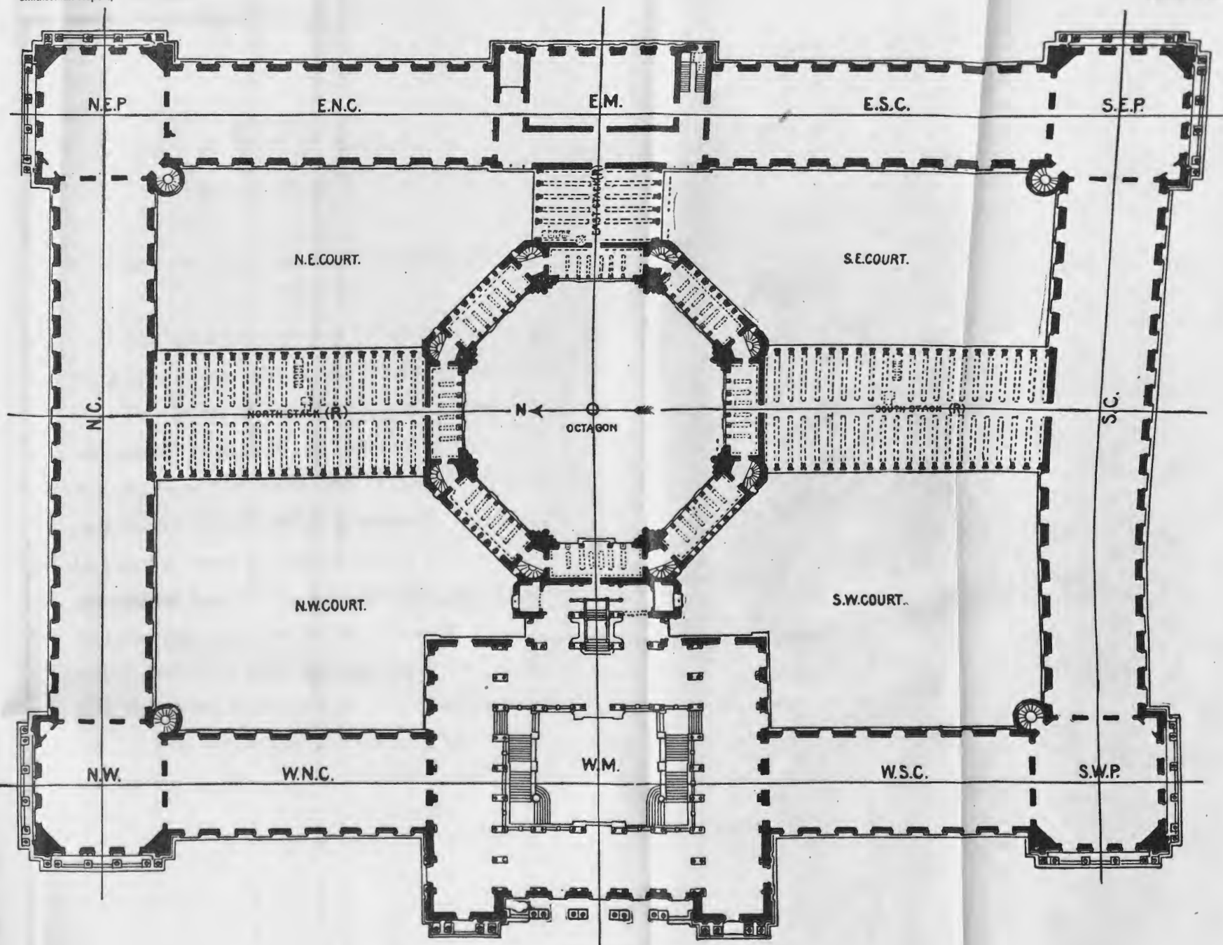
PLAN OF SECOND STORY OF LIBRARY BUILDING.
