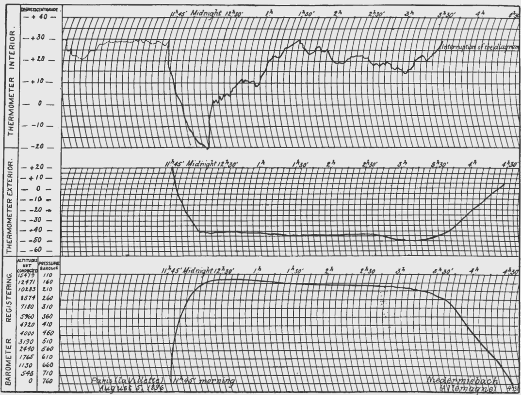
DIAGRAMS OF BALLOON ASCENSIONS OF AUGUST 5, 1896, AT PARIS, FRANCE.
