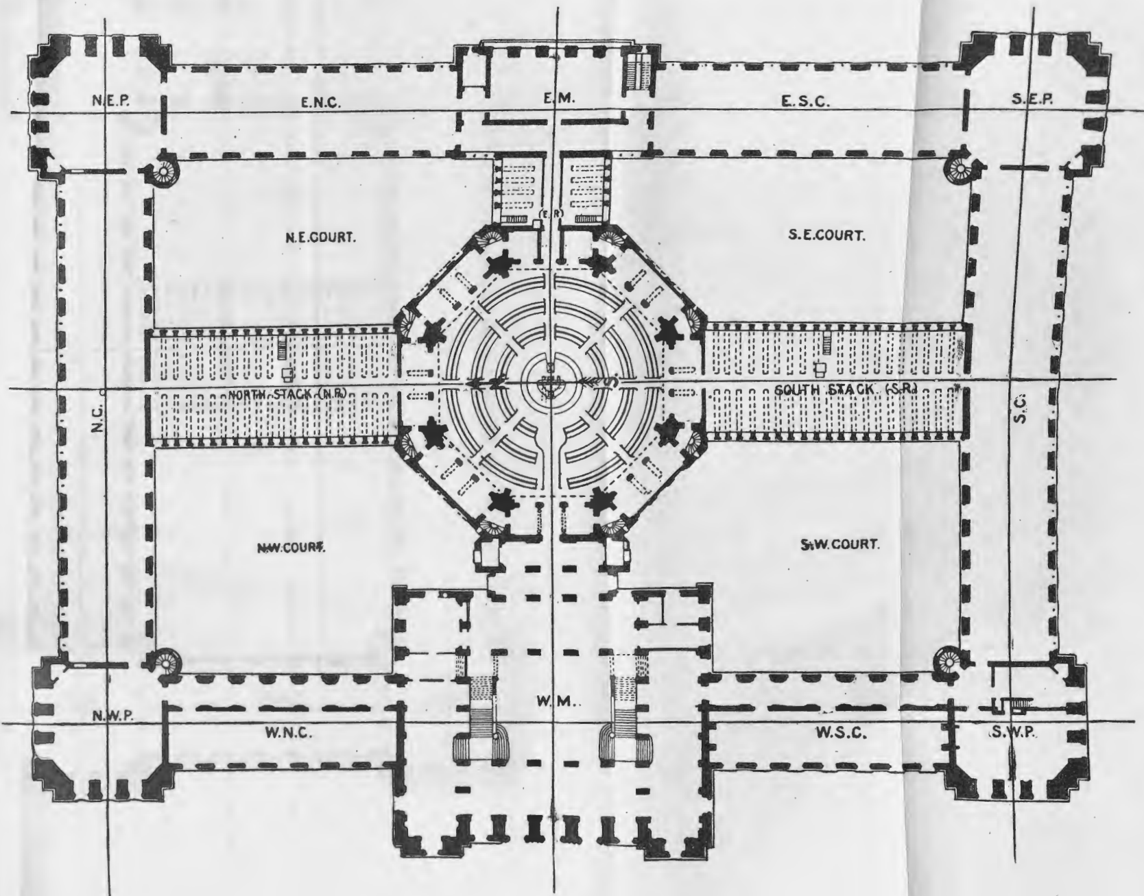
PLAN OF FIRST STORY OF LIBRARY BUILDING.
