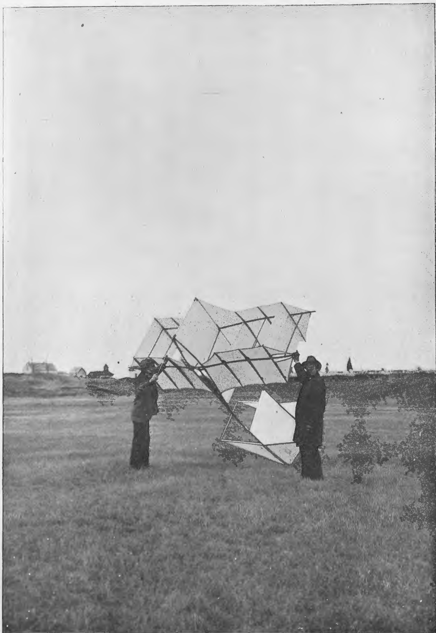
LAMSON'S AERO-CURVE FOLDING KITE.
