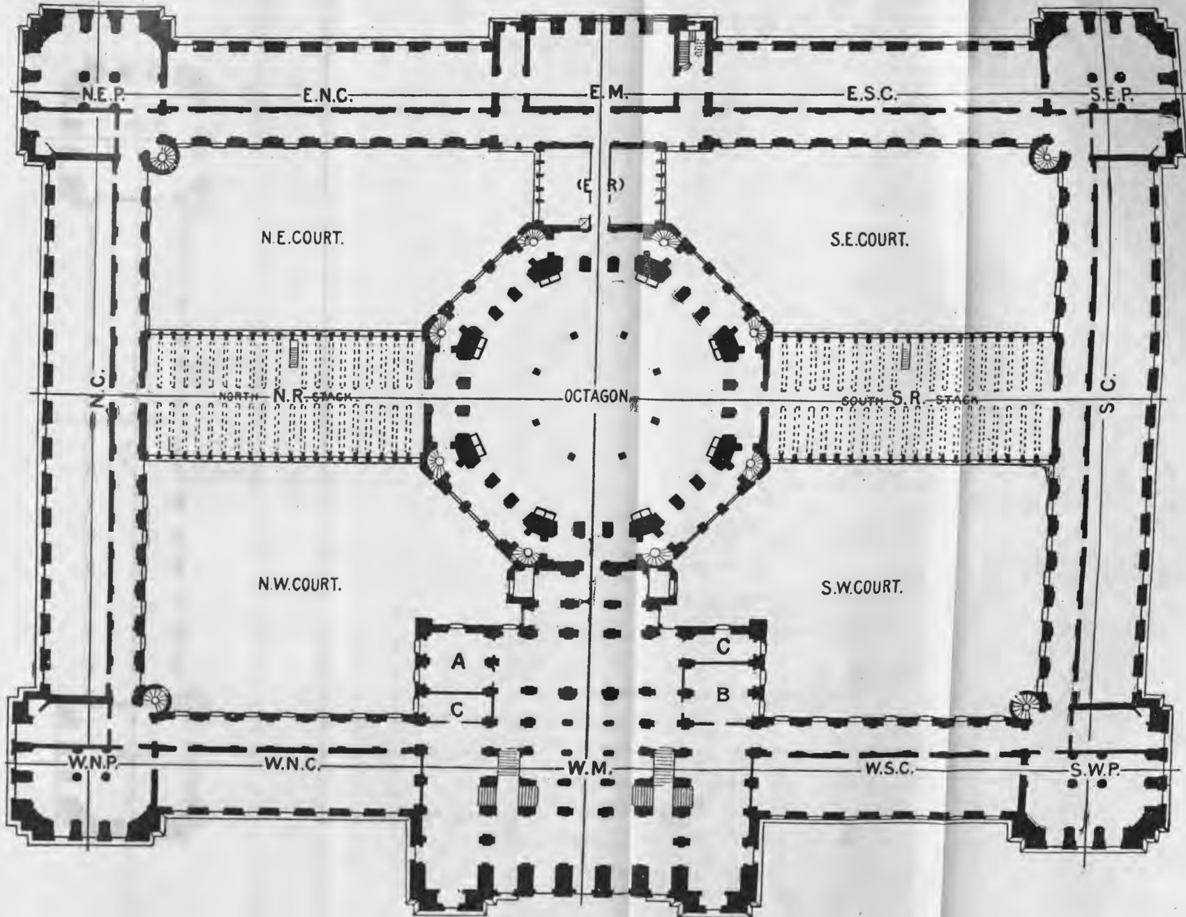
PLAN OF BASEMENT FLOOR OF LIBRARY BUILDING.
