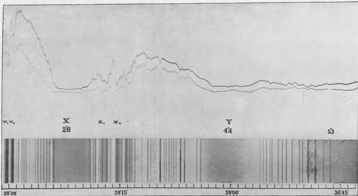
INFRA-RED SOLAR SPECTRUM OF A 60° ROCK-SALT PRISM, b .
