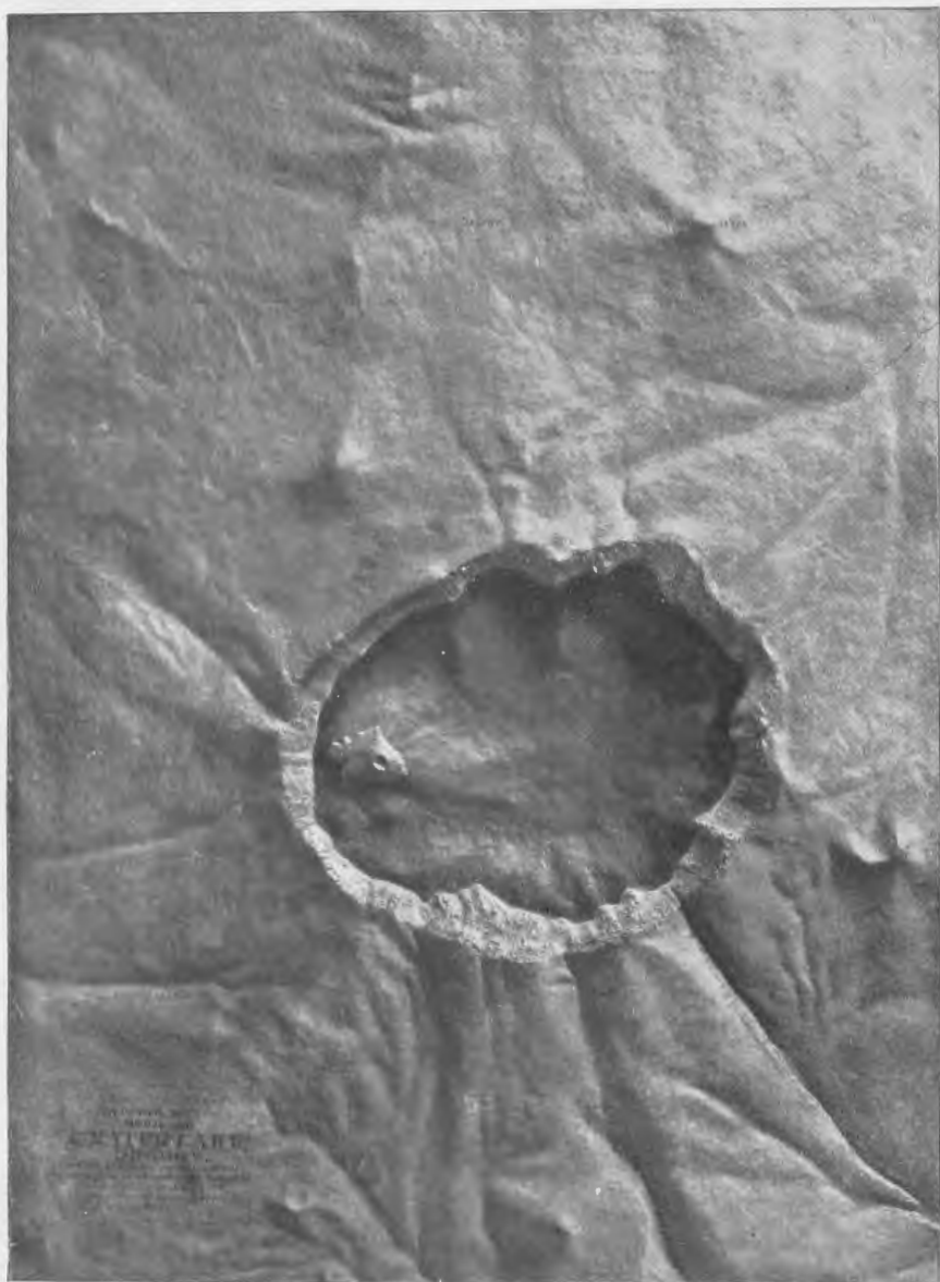
FIG. 15.—CRATER LAKE AS IT WOULD APPEAR FROM A HEIGHT OF OVER 20 MILES ABOVE IT. Prepared from a photograph of a relief model in the U. S. National Museum.
