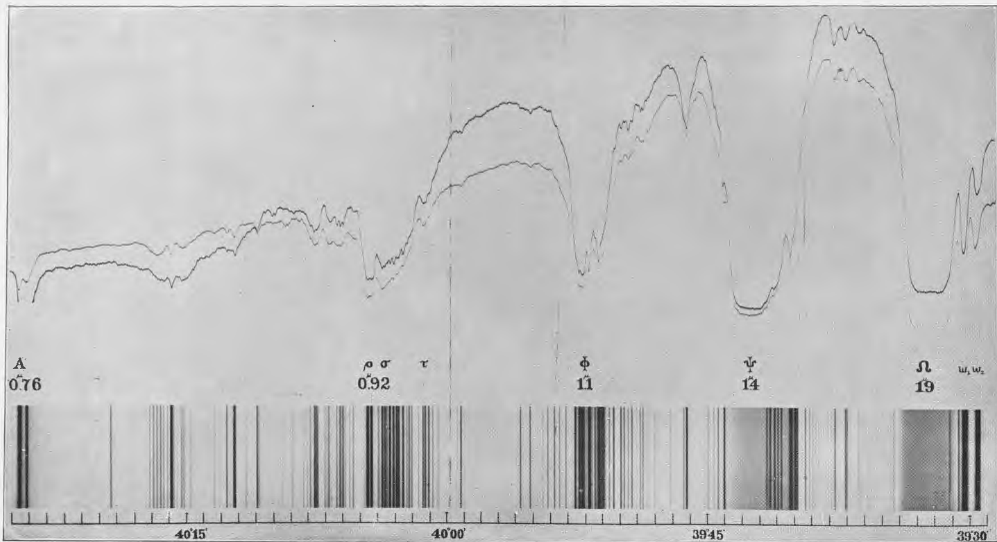
INFRA-RED SOLAR SPECTRUM OF A 60° ROCK-SALT PRISM, a .
