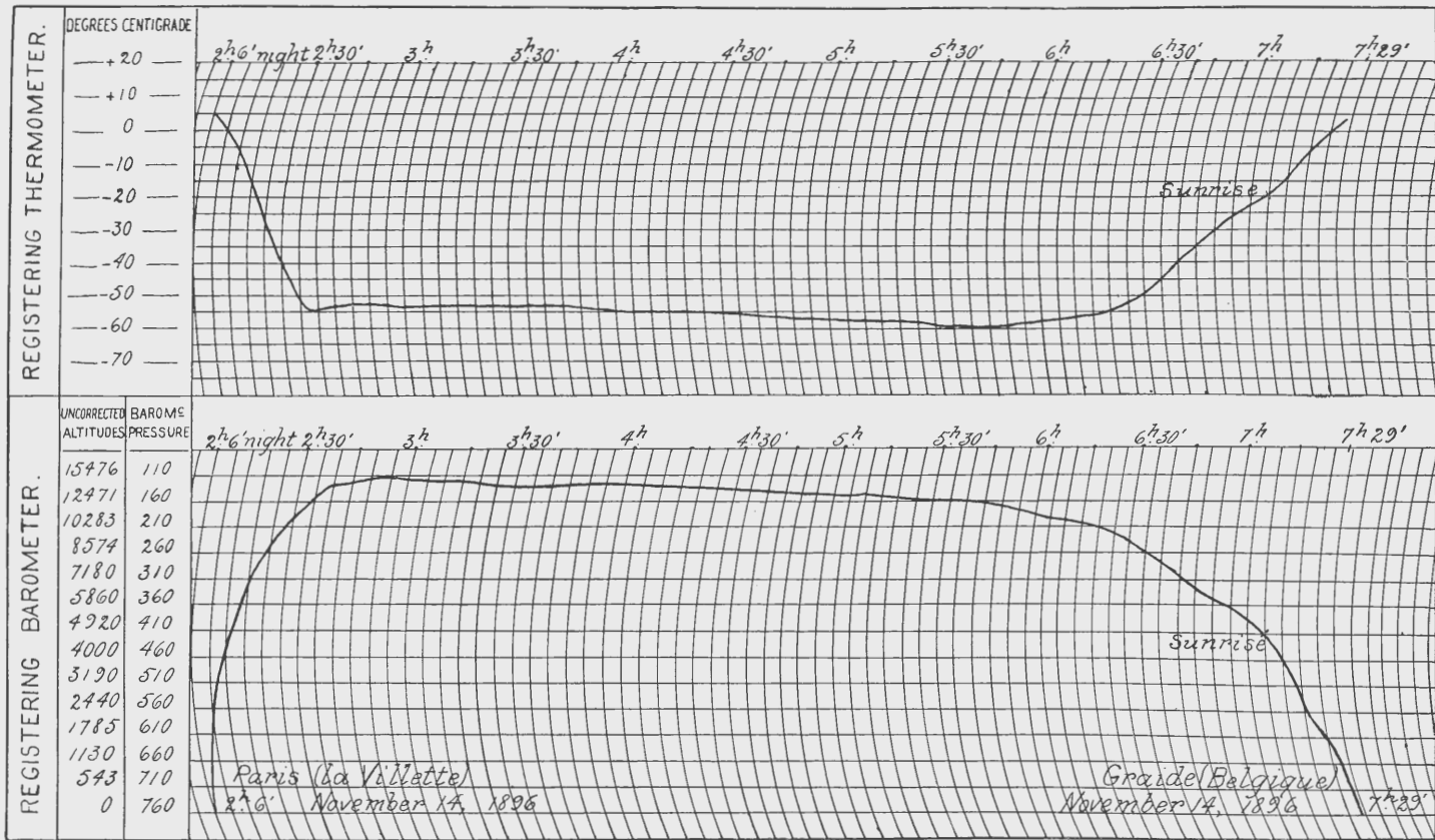
DIAGRAMS OF BALLOON ASCENSIONS OF NOVEMBER 14, 1896, AT PARIS, FRANCE.
