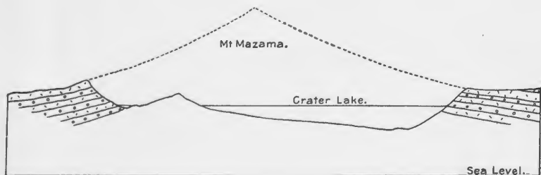
FIG. 9.—SECTION OF CRATER LAKE AND ITS RIM, WITH THE PROBABLE OUTLINE OF MOUNT MAZAMA. STRUCTURAL DETAILS GENERALIZED. Vertical and horizontal scales the same.
