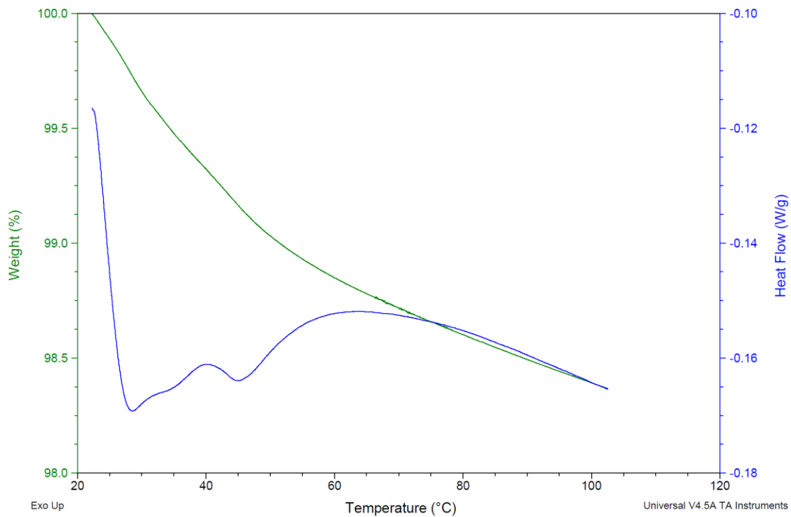
Figure 23: TGA of twice washed 1:6 nano-LAO, vacuum dried, that does not show the characteristic desiccant curves
