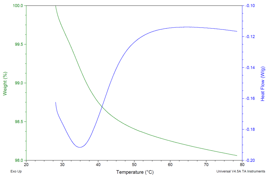
Figure 22: TGA of partially washed 1:6 nano LAO (typical results) showing the inverse peak at 35°C and < 2% desorption
