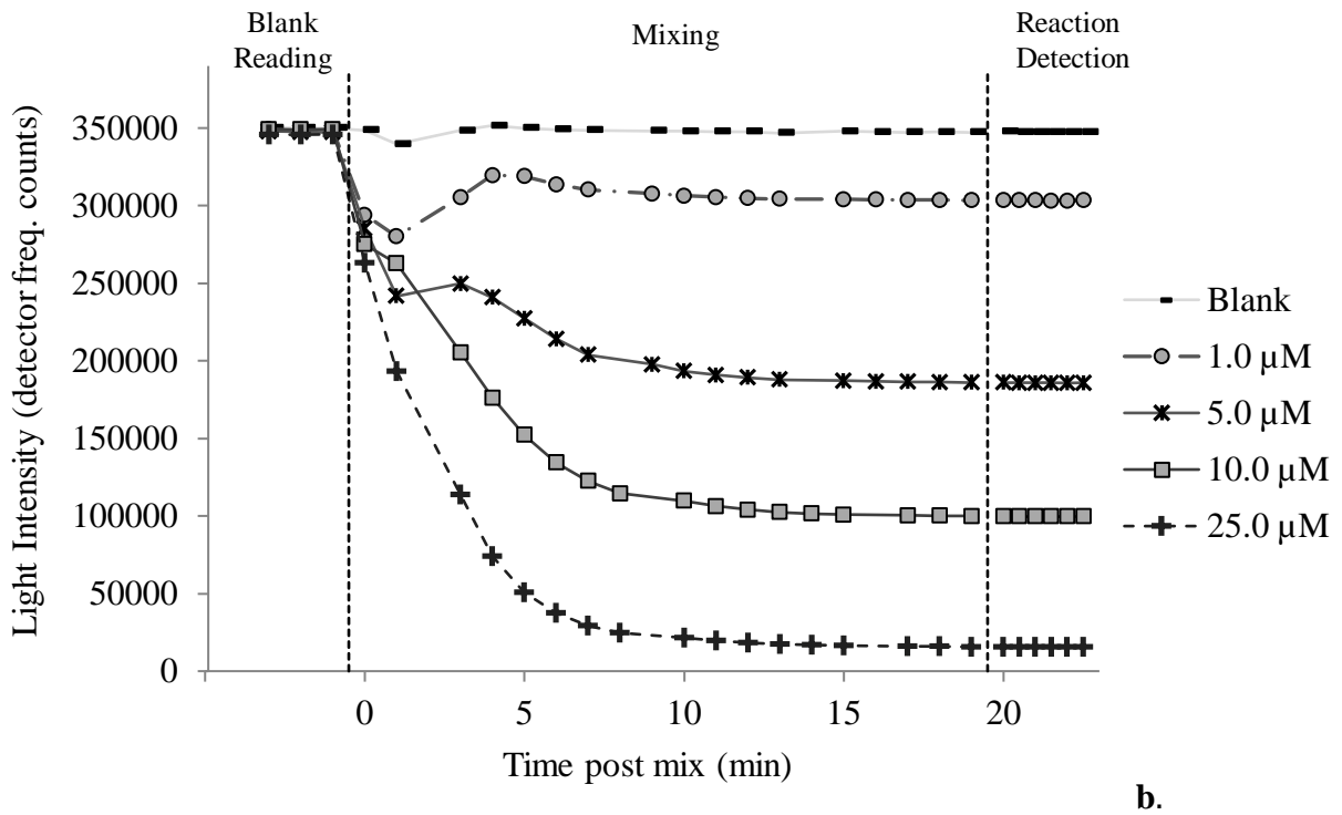
Figure B.7a. Reaction kinetics of Molecular Probes nitrite reagent on prototype nitrite analyzer with 20 mm flow-cell over low range standards and b. over high range standards.
