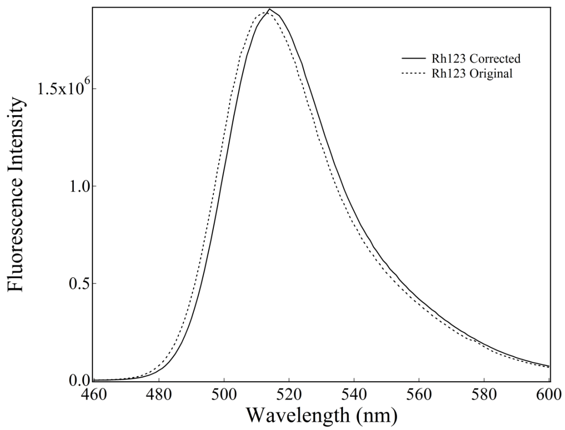
Fig 5.2.1 Uncorrected (dotted line; \lambda_{\text{max}}=512\text{nm} ) and correct (solid line; \lambda_{\text{max}}=514\text{nm} ) fluorescence spectra of Rhodamine 123 in
