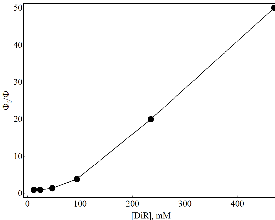
Fig. 4.3.1.7 Classical Stern-Volmer plot for the quenching of DiR fluorescence as a function of dye concentration in the core region of PEG- b -PCL polymeric micelles.
