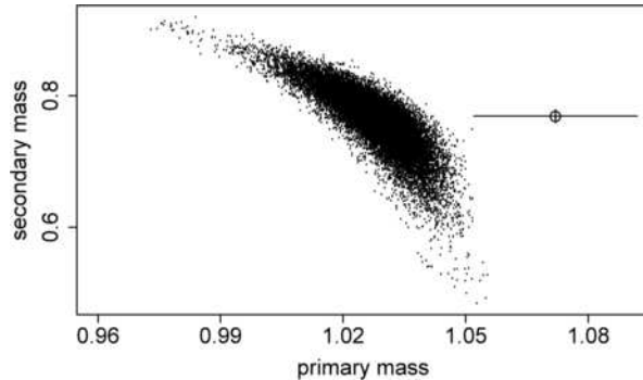
FIG. 5. The Joint Posterior Distribution for the Primary and Secondary Masses of the Star vB022 in the Hyades. The scatter plot shows the Monte Carlo sample from the posterior distribution under our analysis using the Yale–Yonsei model for main sequence evolution. The star has a posterior probability of cluster membership equal to 99.955% and the plot gives the conditional posterior distribution of the two masses given that the binary system is a member of the cluster. This is compared with an external estimate of the two masses that is indicated by the open circle with whiskers that correspond to 95% marginal confidence intervals. Our estimate of the primary mass is about 5% lower than the more reliable external estimate. This difference is attributed to systematic errors in the underlying physical models. The masses are in units of M_{\odot} .
