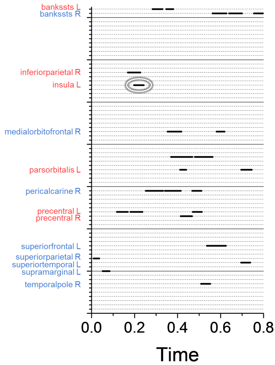
Figure 32. Timecourse of significant differential evoked responses for the Face Trace CS+ > Face Trace CS- comparison. Label color represents the direction of the effect. Circled effects were considered transient and graphed individually below.
