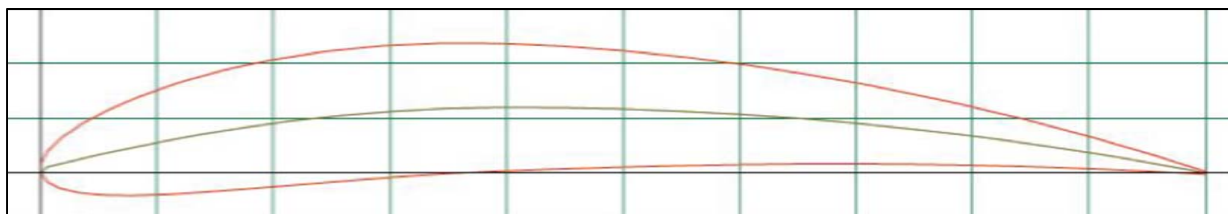
Figure 3. NACA 6412 profile
