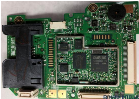
Figure 5. Vx610 Motherboard
