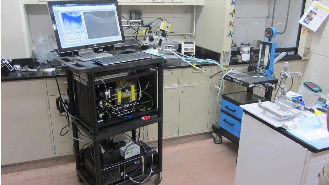
Figure 31 - OCT system during an optogenetic experiment in surgery bay.
