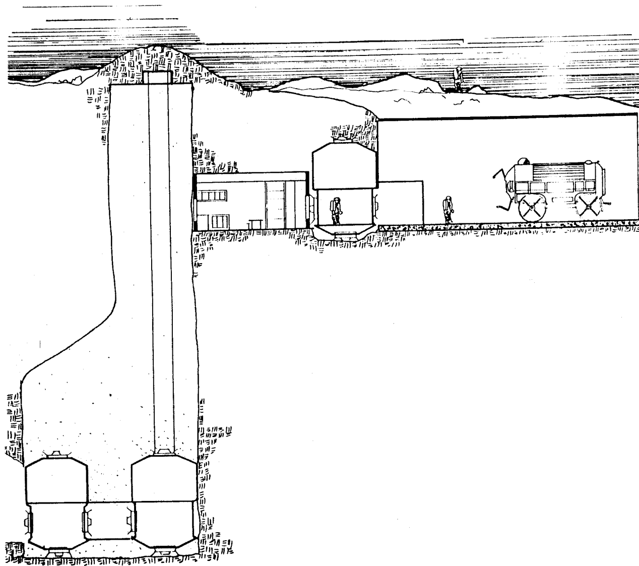
Figure 7.1.2-2. The other entrance/exit to the lava tube showing the logistics/storage area.
