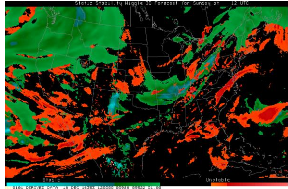
Figure 14c. Experimental Wiggle 3D image of vertical static stability with the enhancement range modified to eliminate more of the unstable image. The transition from orange to red is the adiabatic lapse rate. This allows for one to view the lower levels which show stable air behind the cold front. (See PowerPoint to view the wiggle effect.)
