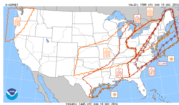
Figure 13b. AIRMETs for turbulence valid for Dec. 18, 2016 15Z. While the areas of wind shear in the eastern US are consistent with the turbulence forecasts, the areas of low level wind
